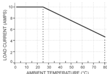
Fig.1 Convection Cooling
