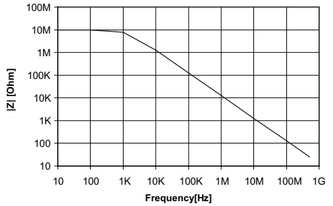
Typical input impedance PMS211A
