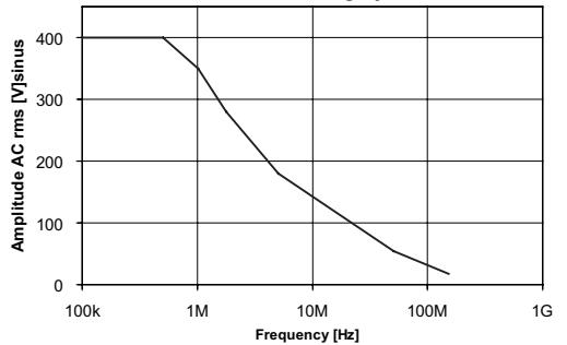
Typical Voltage Derating PMS211A Measurement Category I
