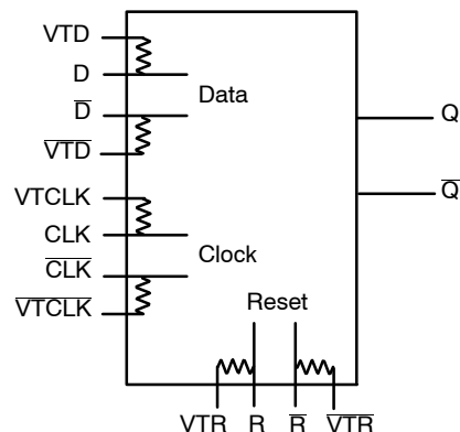
Figure 1. Logic Diagram
