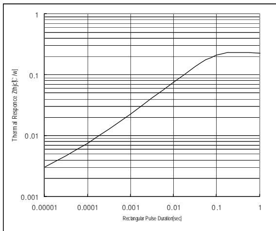
Fig. 3 : Transient Thermal Impedance (Zthjc) Characteristics
