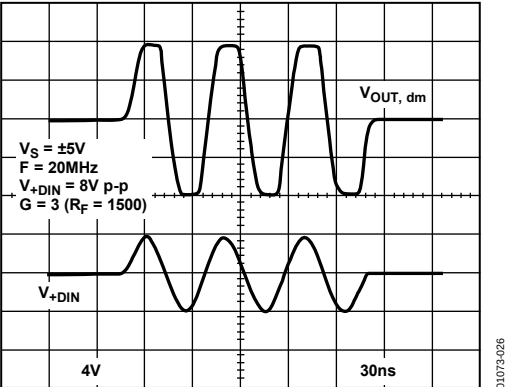
Figure 26. Output Overdrive
