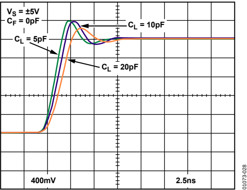
Figure 27. Large Signal Transient Response for Various Cap Loads (See Figure 40)
