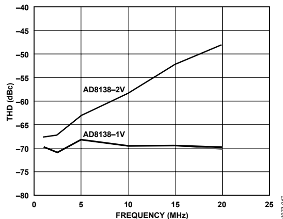
Figure 48. AD9203 THD @ -0.5\ \text{dBFS} AD8138
