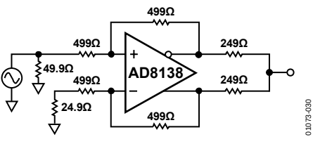
Figure 41. Test Circuit for Output Balance
