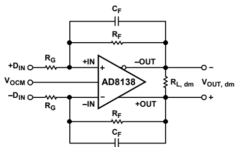
Figure 42. Circuit Definitions
