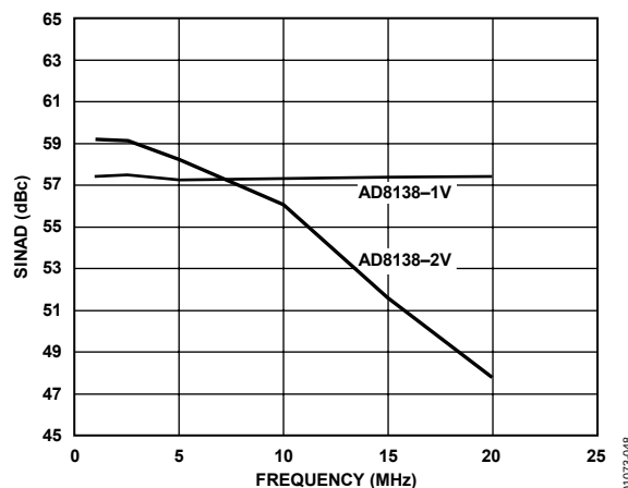
Figure 49. AD9203 SINAD @ -0.5\ \text{dBFS} AD8138
