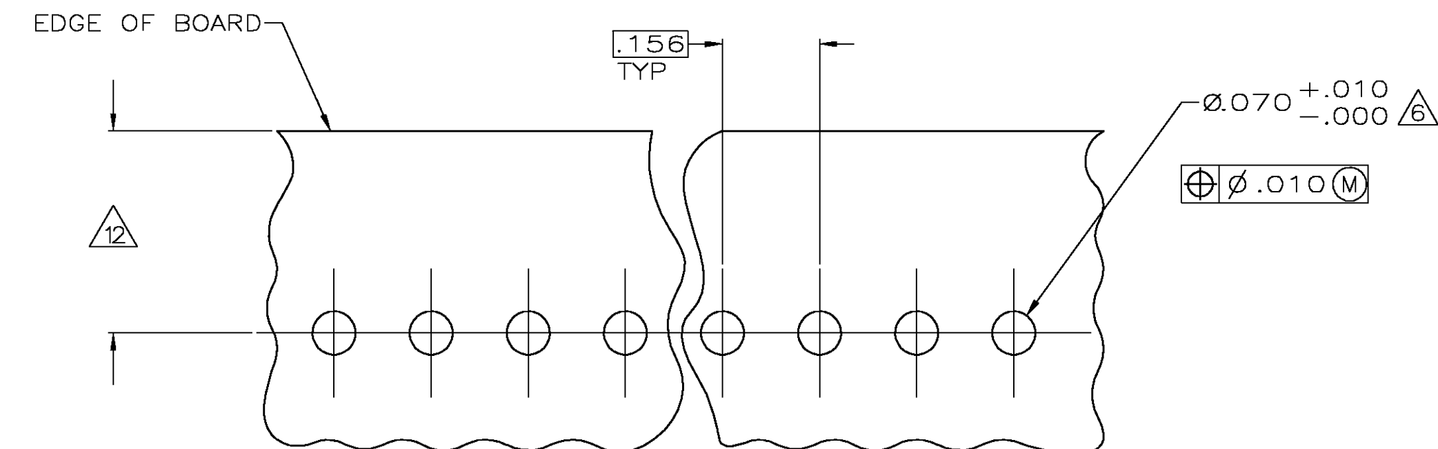
RECOMMENDED MOUNTING HOLE PATTERN FOR .063 THICK P.C. BOARD (feature 2)
