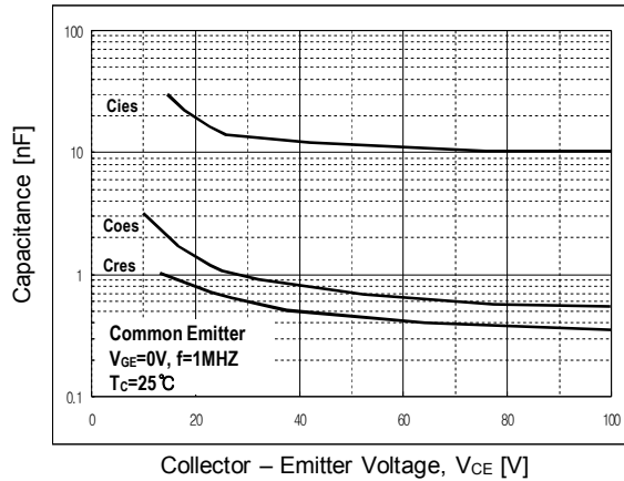
Fig 7. Capacitance characteristics
