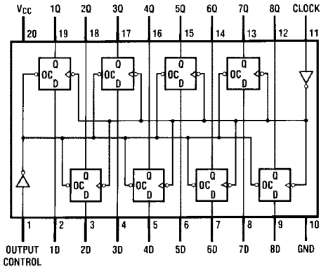
Top View MM74HCT574
