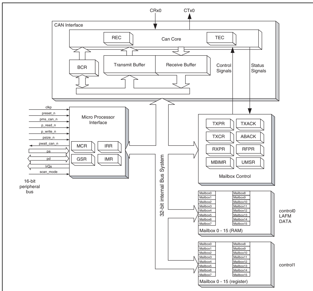
Figure 21.1 RCAN-ET Architecture
