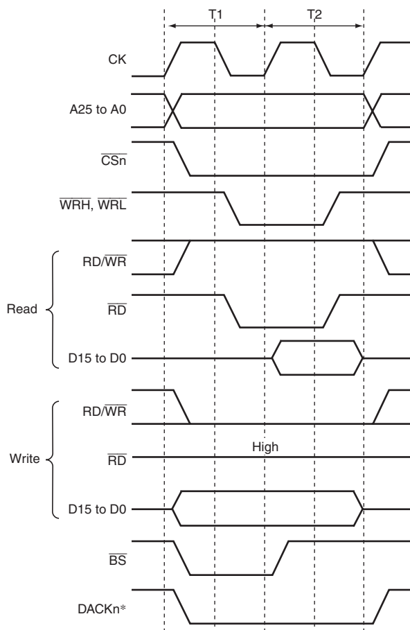
Figure 9.36 Basic Access Timing for SRAM with Byte Selection (BAS = 0)
