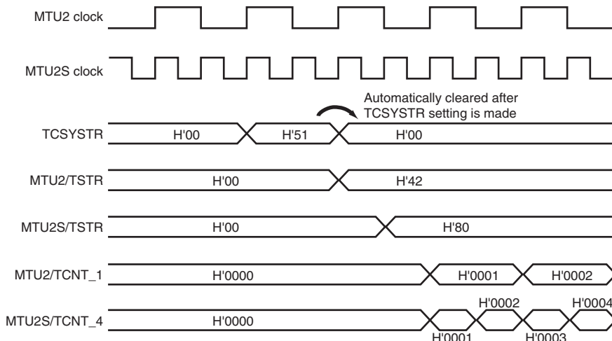
Figure 11.84 (2) Example of Synchronous Counter Start Operation (MTU2-to-MTU2S Clock Frequency Ratio = 1:2)
