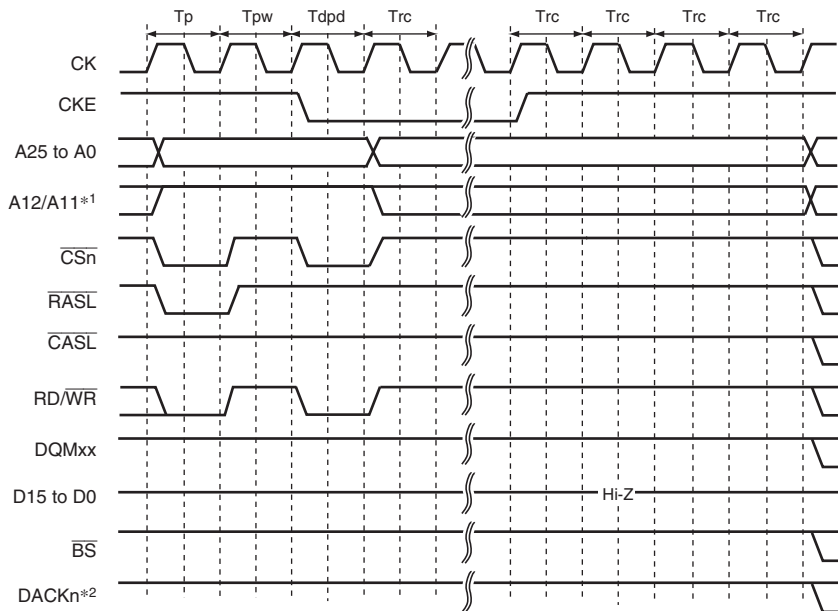
Figure 9.34 Deep Power-Down Mode Transition Timing
