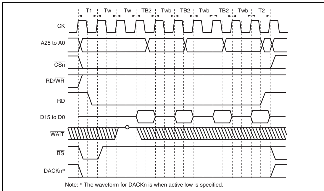
Figure 9.35 Burst ROM Access Timing (Clock Asynchronous)
