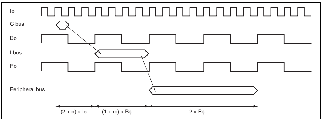
Figure 9.44 Timing of Write Access to On-Chip Peripheral I/O Registers When I\phi:B\phi:P\phi = 4:1:1
