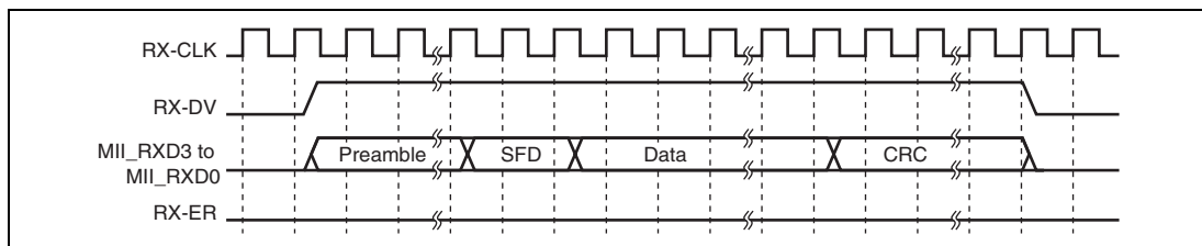
Figure 25.4 (4) MII Frame Receive Timing (Normal Reception)
