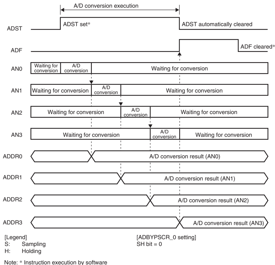
Figure 20.3 Example 2 of A/D_0 Converter Operation (Single-Cycle Scan Mode and Sample-and-Hold Circuit Disabled)
