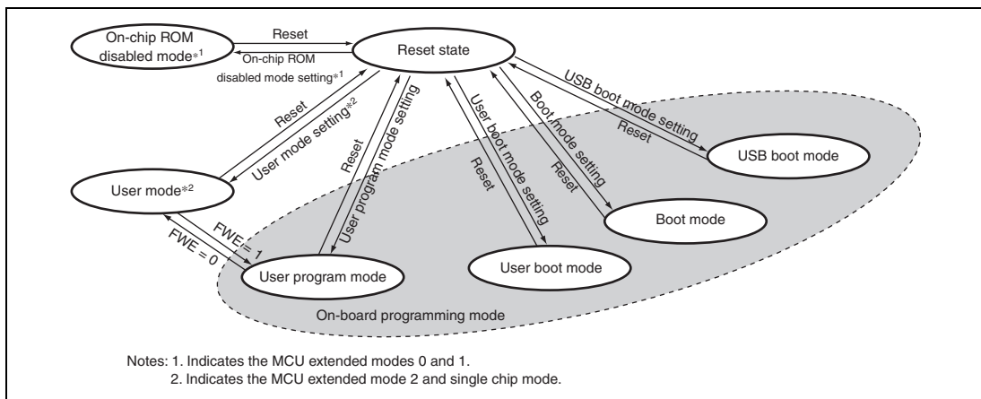
Figure 28.4 FLD-Related Mode Transition
