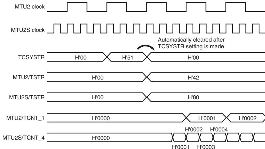
Figure 11.84 (3) Example of Synchronous Counter Start Operation (MTU2-to-MTU2S Clock Frequency Ratio = 1:3)
