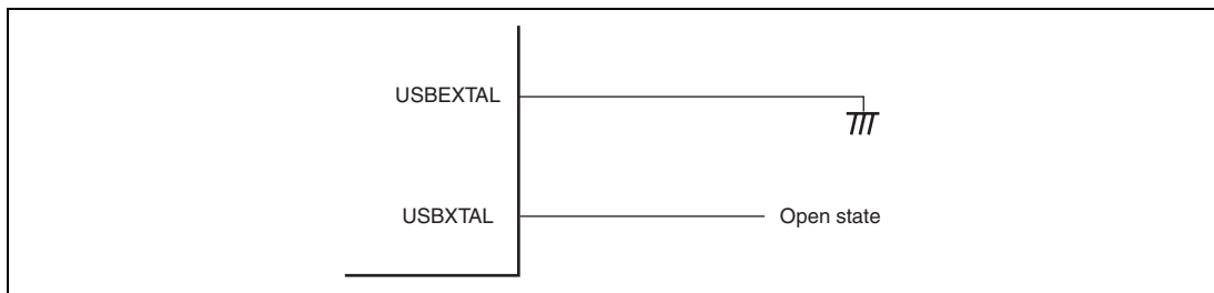
Figure 4.8 Handling of Pins when a Ceramic Resonator is not Connected
