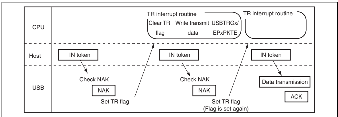
Figure 24.29 Timing for Setting the TR Interrupt Flag
