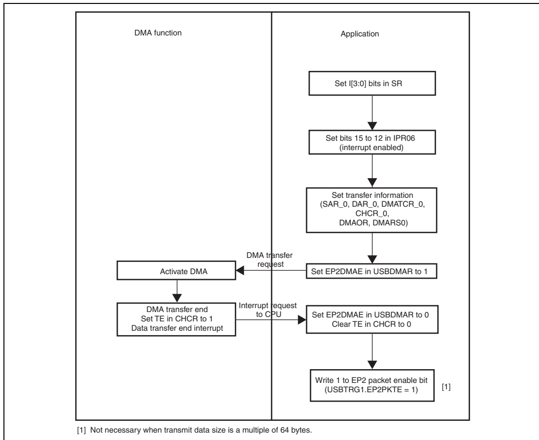
Figure 24.20 Example of DMA Transfer (Channel 0) for Bulk-IN Transfer (EP2) (When Transmit Data Size is Determined Before Receiving IN Token)
