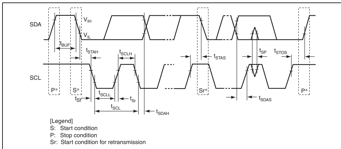
Figure 33.55 I²C Bus Interface 3 Input/Output Timing
