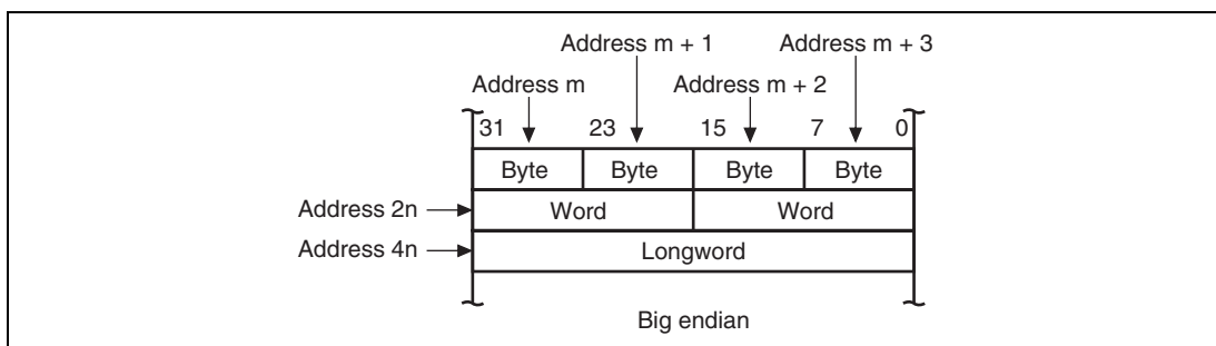
Figure 2.7 Data Formats in Memory
