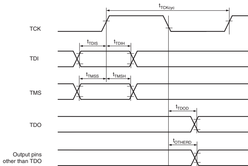
Figure 33.67 H-UDI Data Transmission Timing
