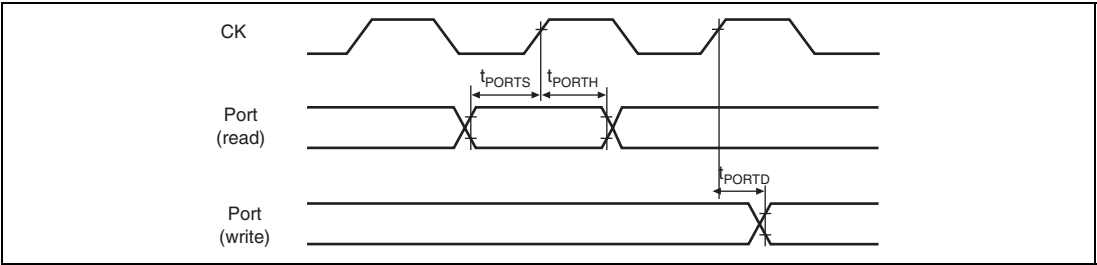
Figure 33.57 I/O Port Timing
