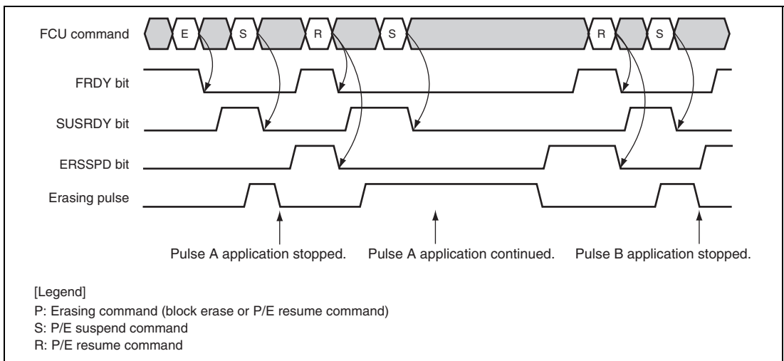
Figure 27.32 Suspending Erasure Processing (Suspension-Priority Mode)
