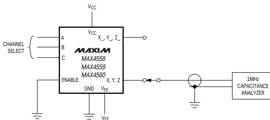
Figure 5. Channel Off/On-Capacitance
