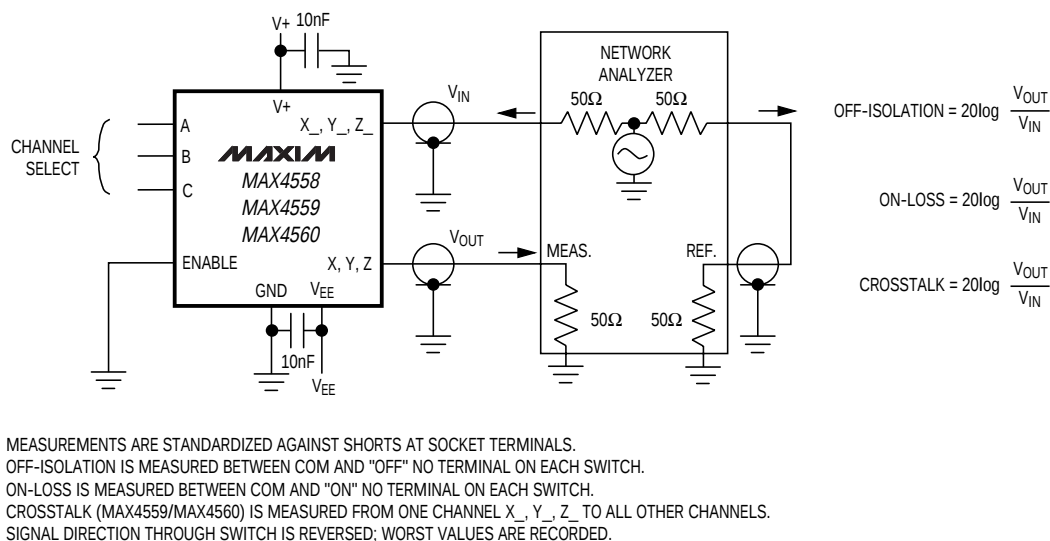
Figure 4. Off-Isolation/On-Channel Bandwidth and Crosstalk
