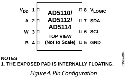
Figure 4. Pin Configuration
