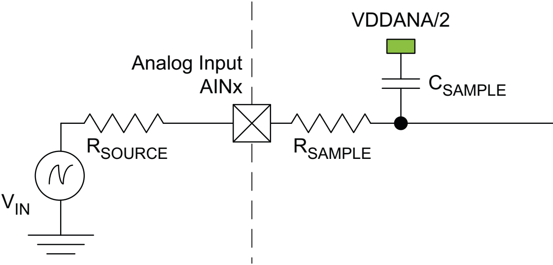
Figure 36-3. ADC Input
