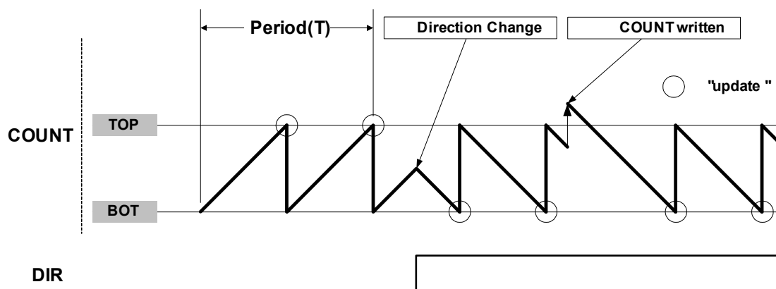
Figure 29-3. Counter Operation
