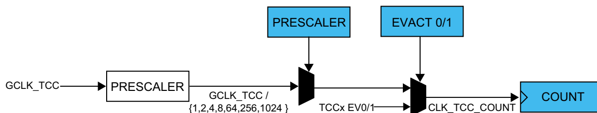
Figure 30-4. Prescaler
