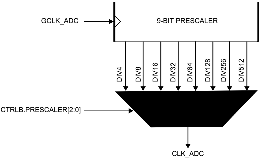
Figure 32-2. ADC Prescaler
