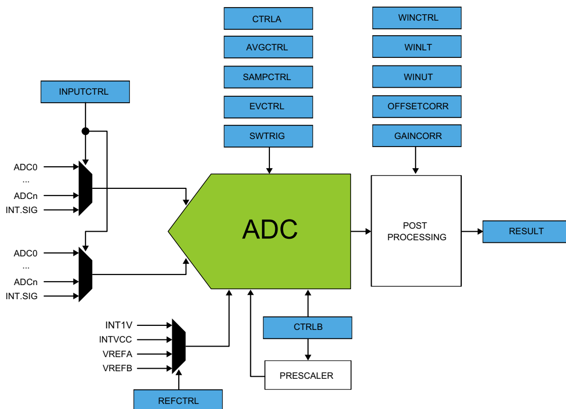
Figure 32-1. ADC Block Diagram
