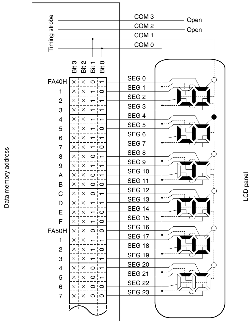
Figure 18-24. Example of Connecting Two-Time-Slice LCD Panel
