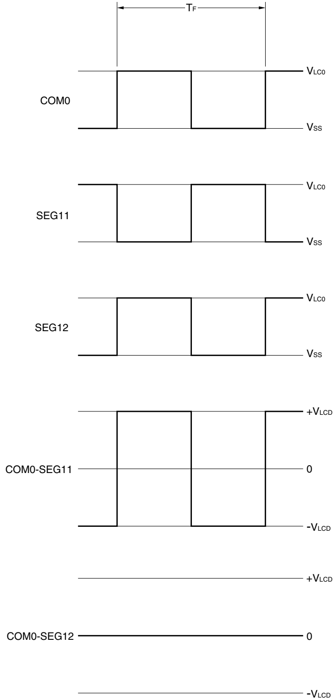
Figure 18-22. Static LCD Drive Waveform Examples
