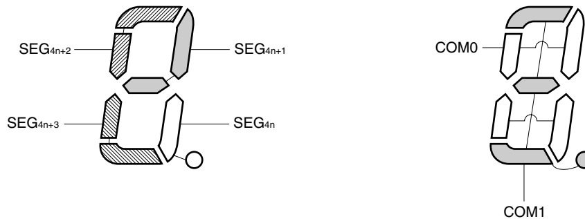
Figure 18-23. Two-Time-Slice LCD Display Pattern and Electrode Connections
