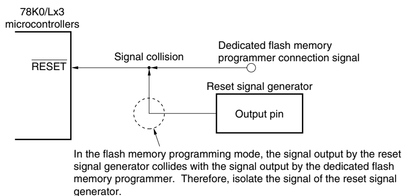
Figure 28-9. Signal Collision ( \overline{\text{RESET}} Pin)
