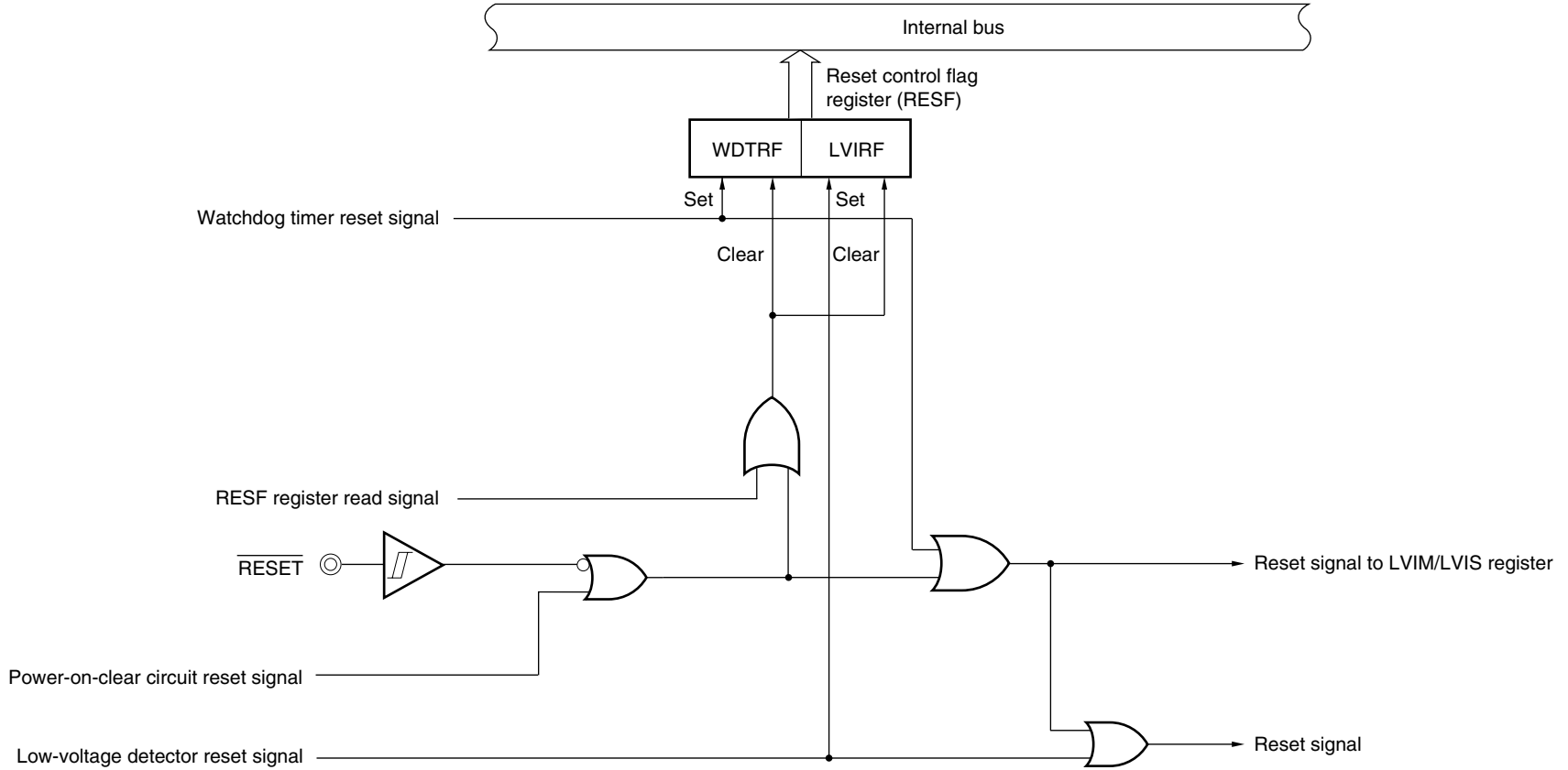
Figure 24-1. Block Diagram of Reset Function
