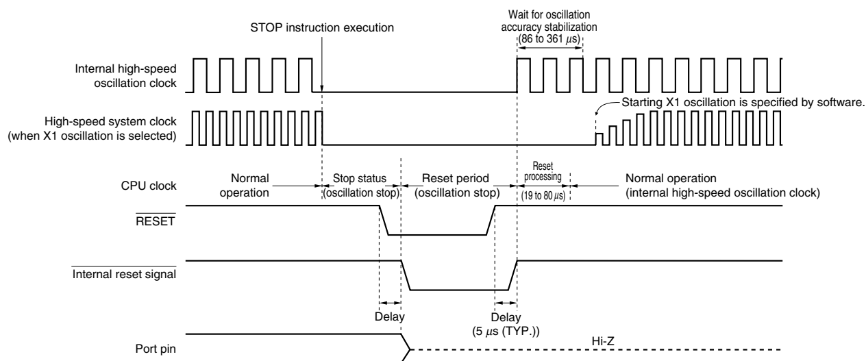
Figure 24-4. Timing of Reset in STOP Mode by RESET Input
