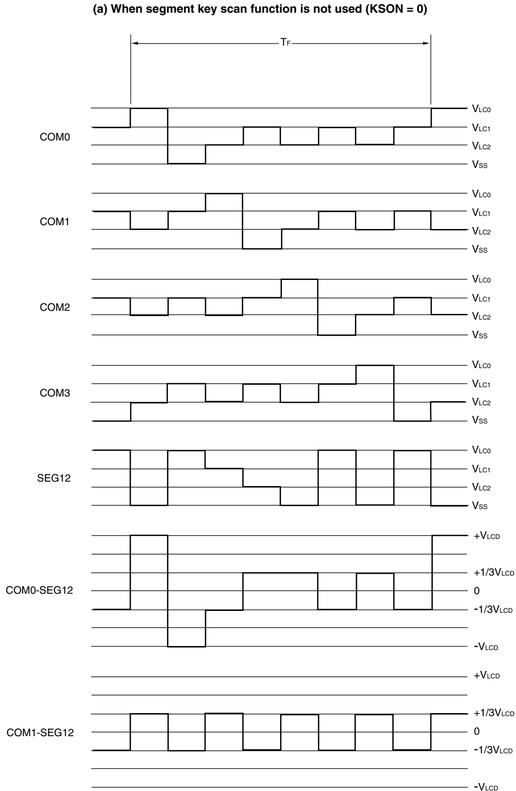
Figure 18-32. Four-Time-Slice LCD Drive Waveform Examples (1/3 Bias Method)
