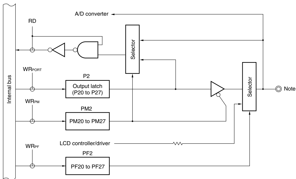
Figure 4-7. Block Diagram of P20 to P27
