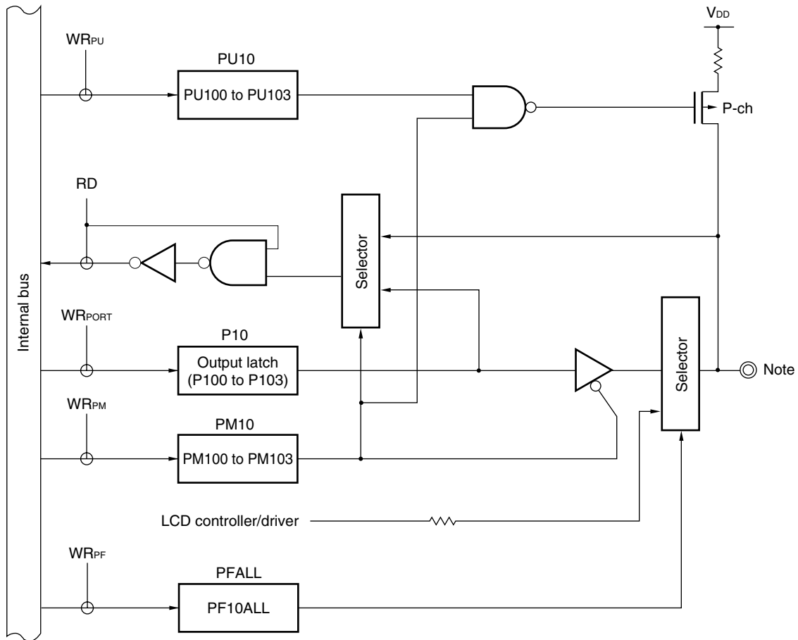
Figure 4-16. Block Diagram of P100 to P103
