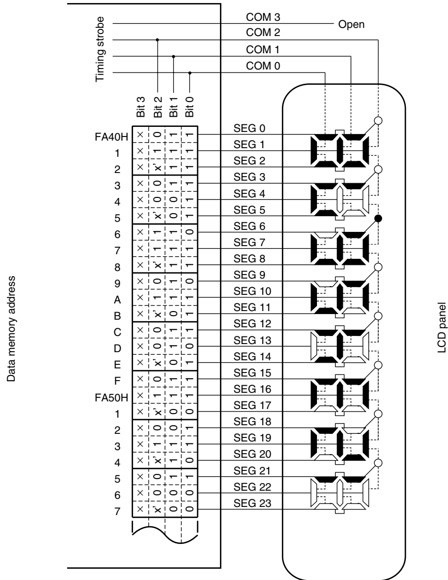
Figure 18-27. Example of Connecting Three-Time-Slice LCD Panel
