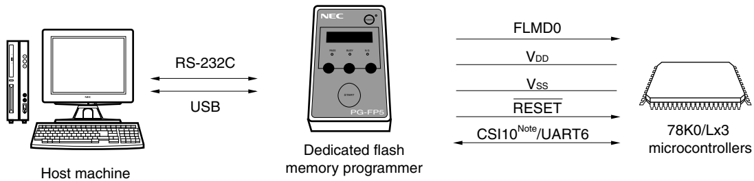
Figure 28-3. Environment for Writing Program to Flash Memory
