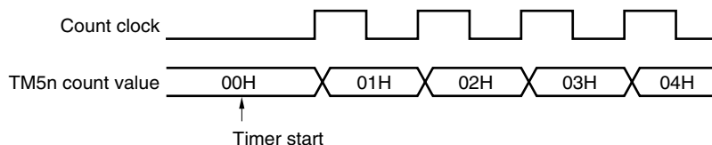
Figure 7-20. 8-Bit Timer Counter 5n (TM5n) Timing
