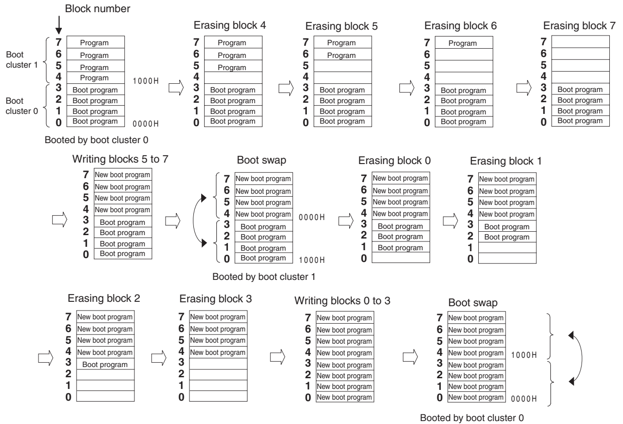
Figure 28-16. Example of Executing Boot Swapping
