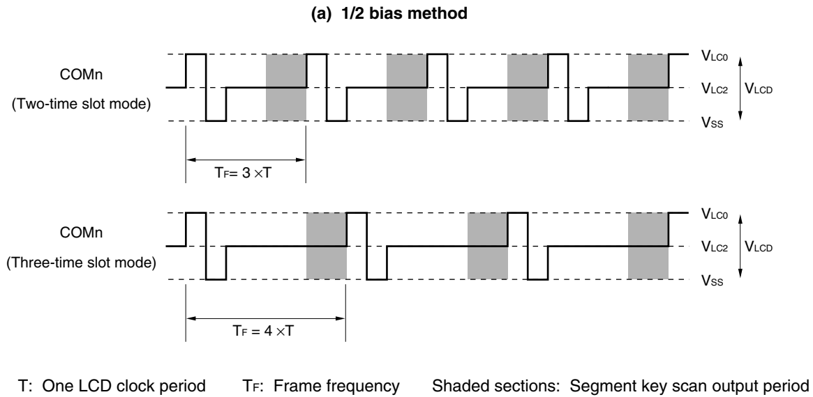
Figure 18-18 Common Signal Waveforms
