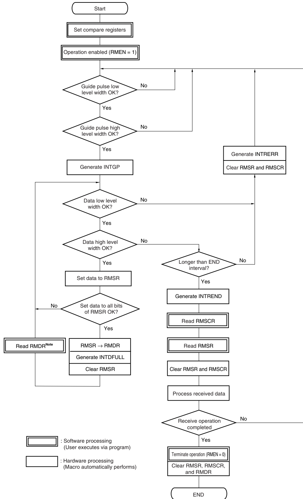
Figure 20-9. Operation Flow of Type B Reception Mode
