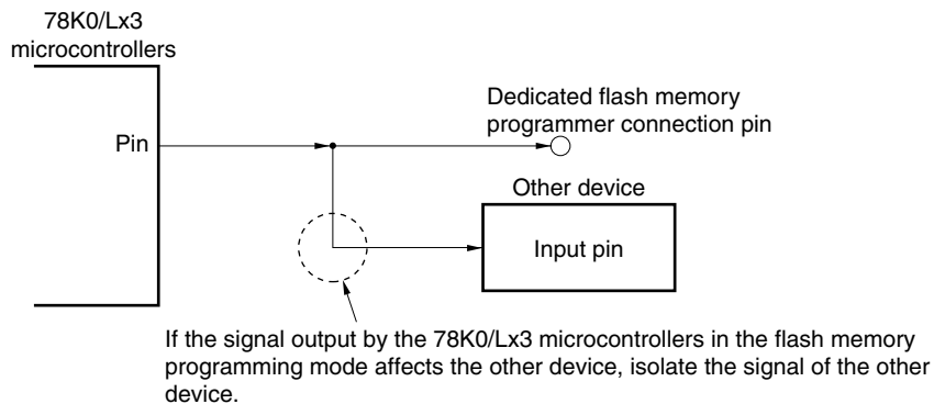
Figure 28-8. Malfunction of Other Device
