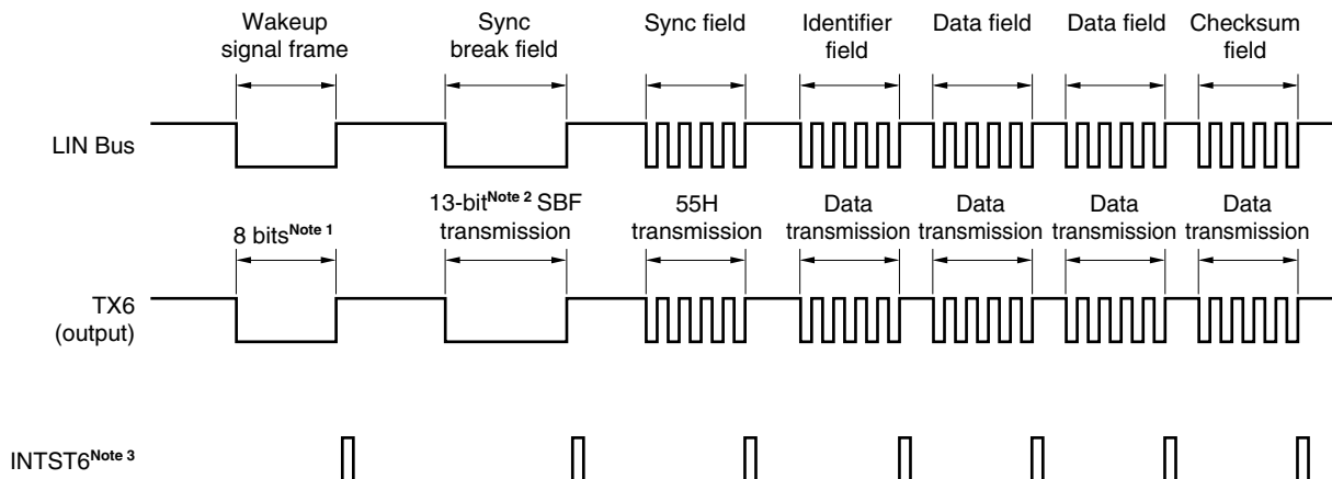
Figure 15-1. LIN Transmission Operation
