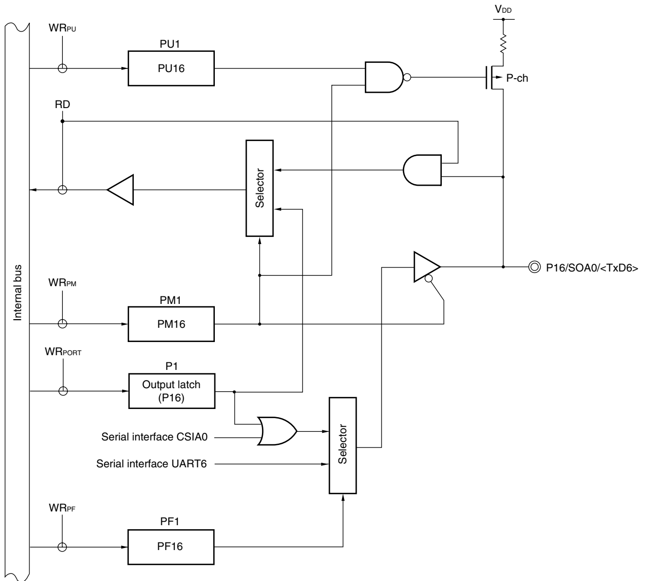
Figure 4-5. Block Diagram of P16
