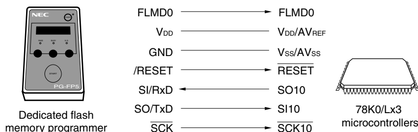
Figure 28-4. Communication with Dedicated Flash memory programmer (CSI10)
