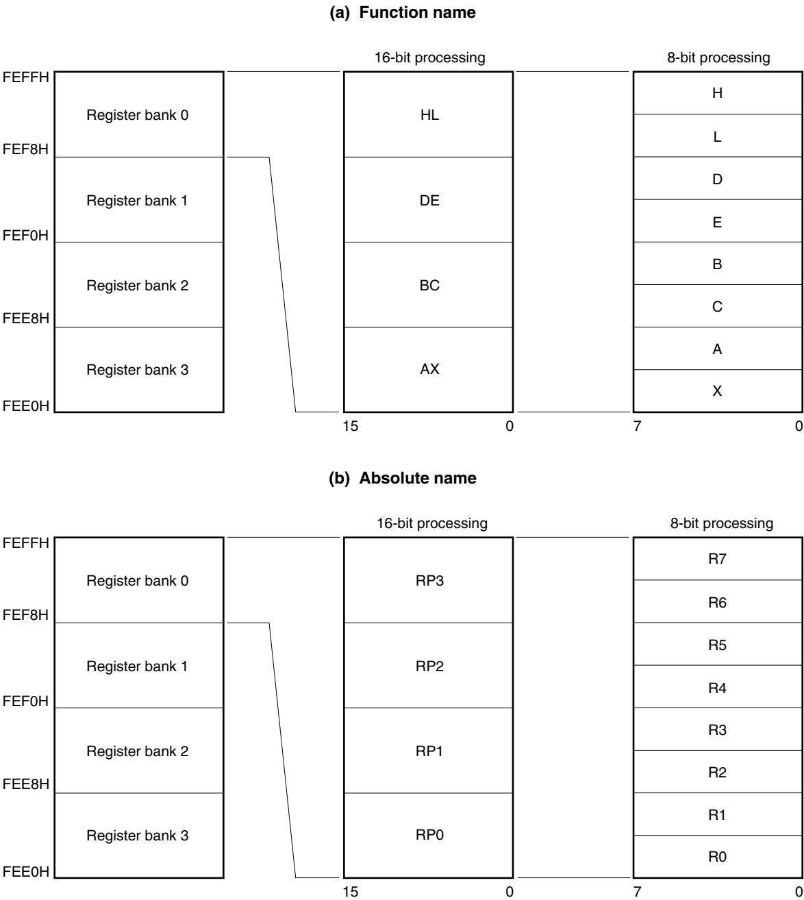
Figure 3-18. Configuration of General-Purpose Registers
