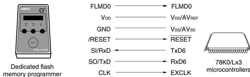
Figure 28-5. Communication with Dedicated Flash memory programmer (UART6)
