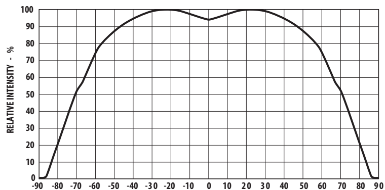
Figure 7. Relative intensity vs. angle for HSMW-C191.
