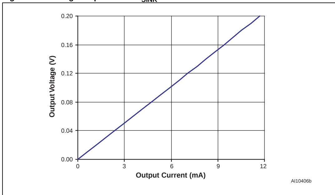
Figure 17. Voltage output low vs. I_{SINK}
