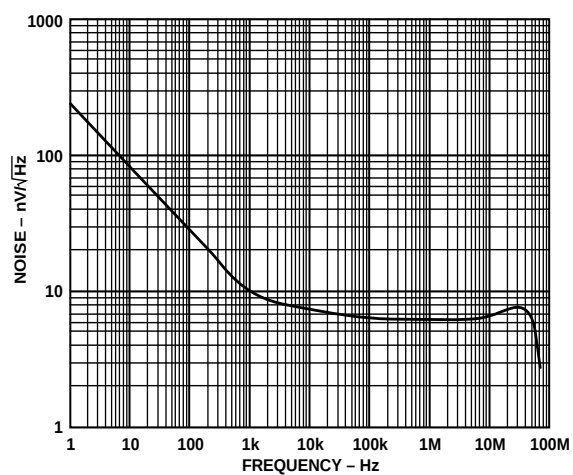
Figure 24. Voltage Noise
