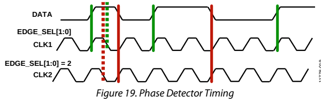
Figure 19. Phase Detector Timing
