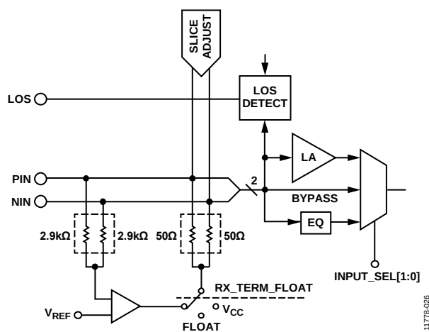
Figure 26. Input Stage Circuit Block Diagram
