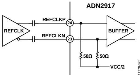
Figure 25. AC-Coupled, Differential REFCLKx Configuration
