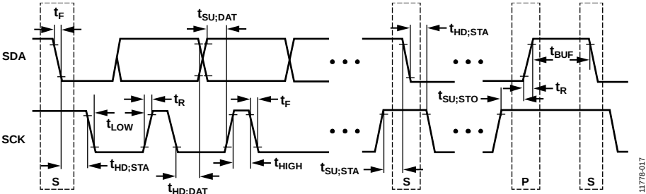
Figure 17. I 2 C Interface Timing Diagram
