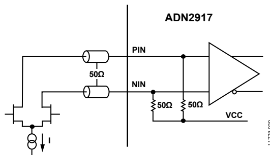
Figure 30. DC-Coupled Application, 0 dB EQ Input (Normal Mode)
