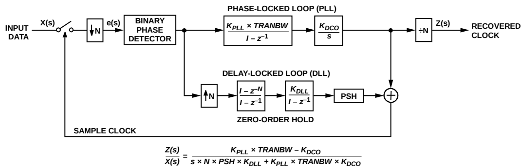
Figure 18. CDR Jitter Block Diagram
