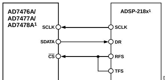
Figure 29. Interfacing to the ADSP-218x
