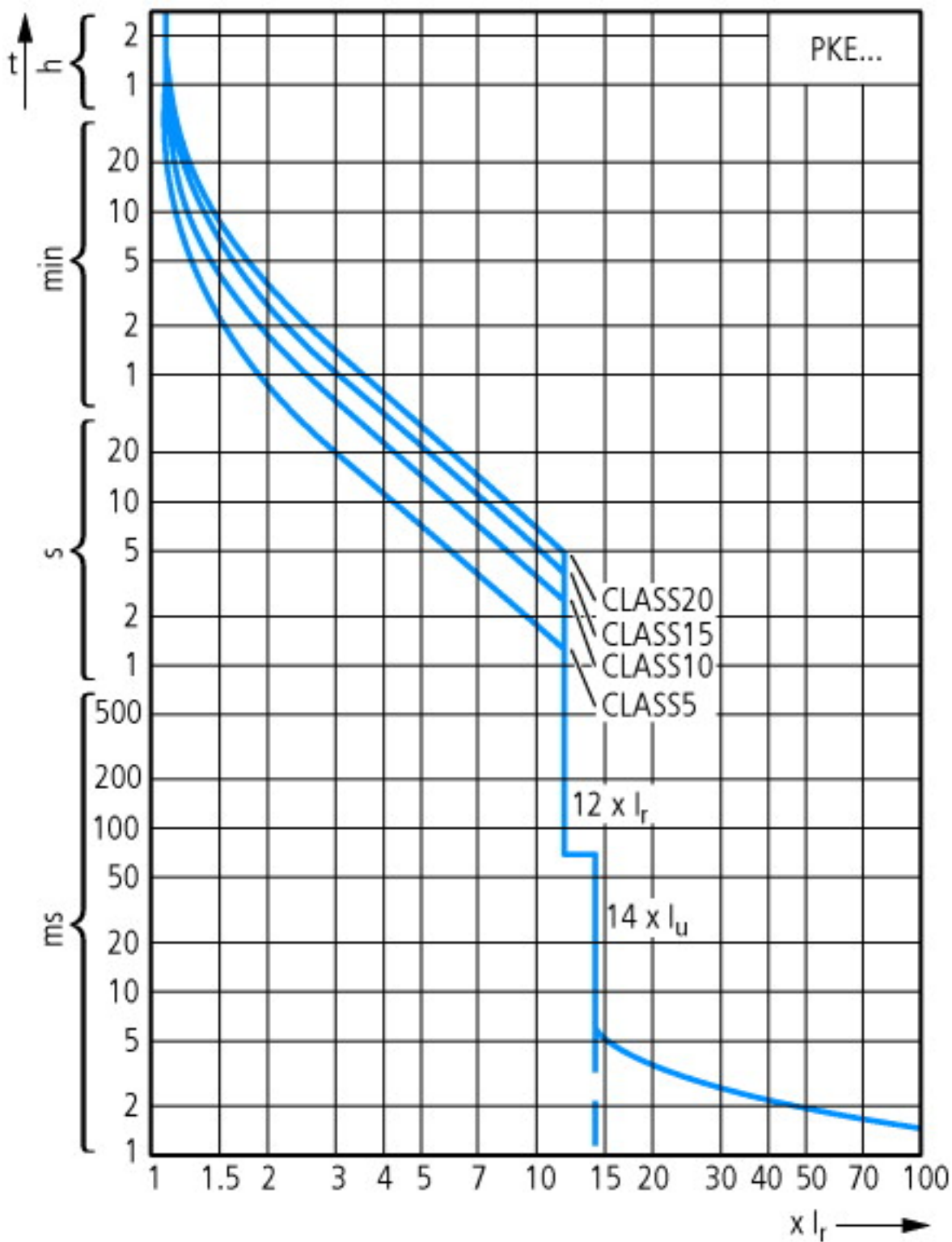
Tripping characteristics
