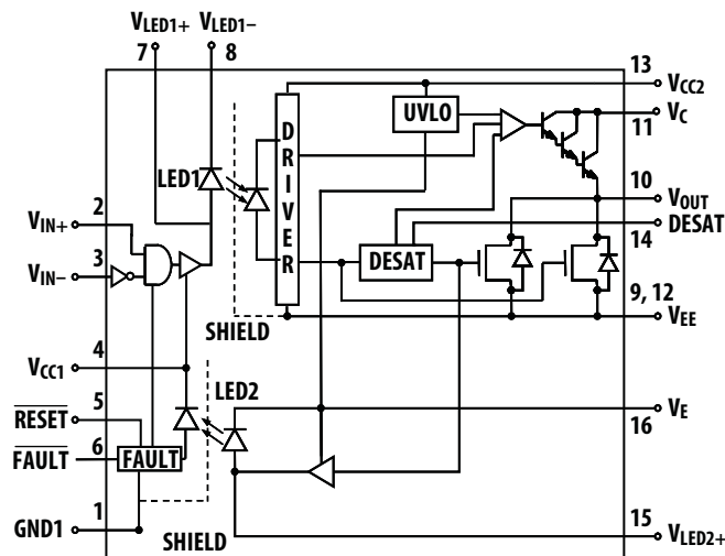
Figure 1. ACPL-38JT Functional Diagram
