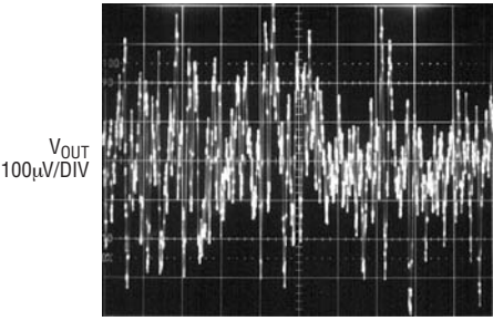
10Hz to 100kHz Output Noise C_{BYP} = 0pF
