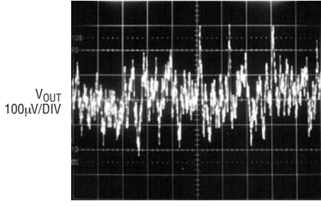
10Hz to 100kHz Output Noise C_{BYP} = 100pF
