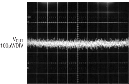
10Hz to 100kHz Output Noise C_{BYP} = 0.01\mu F
