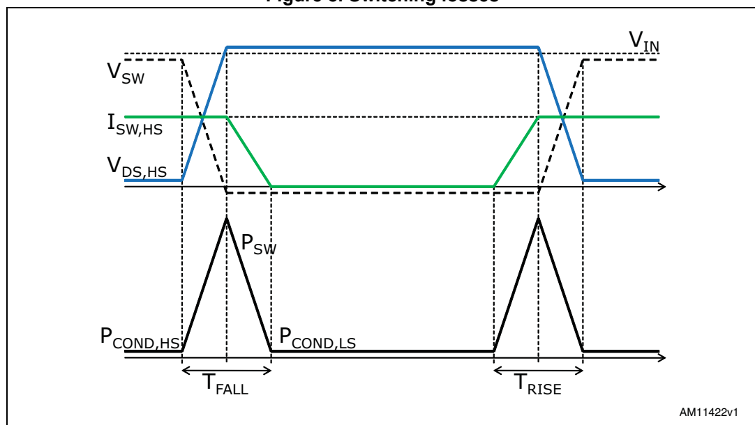
Figure 8. Switching losses
