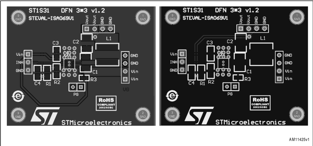
Figure 11. Demonstration board PCB top and bottom, DFN package
