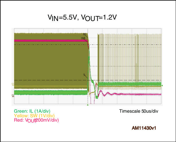
Figure 18. Short-circuit protection
