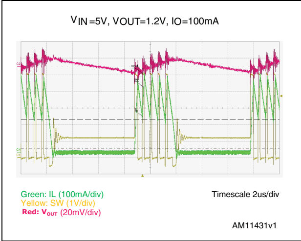
Figure 17. 100 mA operation
