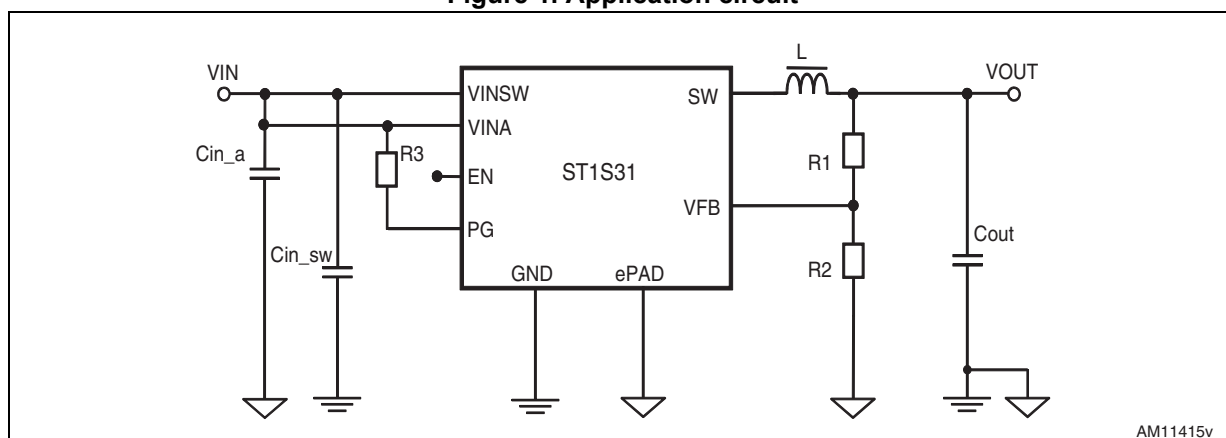
Figure 1. Application circuit
