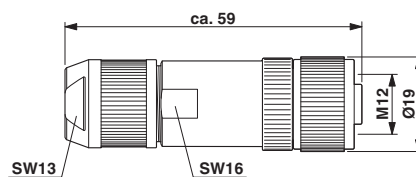
M12 x 1 socket, straight
