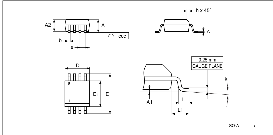
Figure 31. SO8 – 8-lead plastic small package outline
