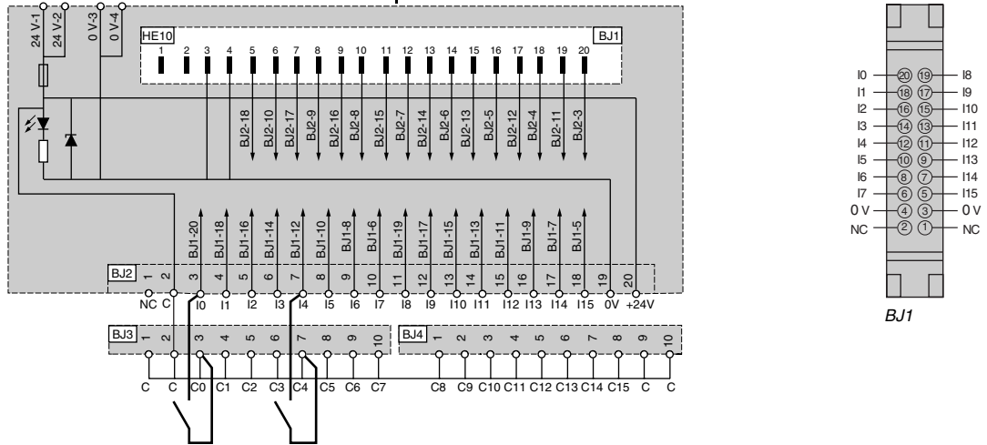
(1) Example of output connections. When connecting an inductive load, include a diode or a varistor.
