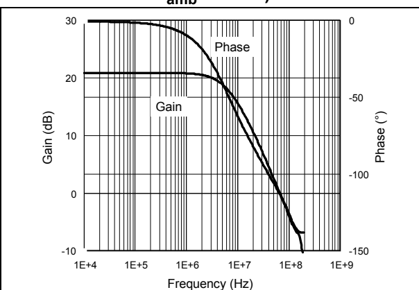
Figure 35. Closed loop gain and phase vs. frequency (gain = +11, V_{CC} = \pm 5\text{ V} , R_L = 150\ \Omega , T_{amb} = 25\text{ }^\circ\text{C} )
