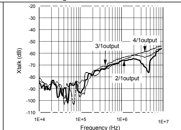
Figure 41. Channel separation (Xtalk) vs. frequency (gain = +11, V_{CC} = \pm 5\text{ V} , Z_L = 150\ \Omega // 27\text{ pF} )
