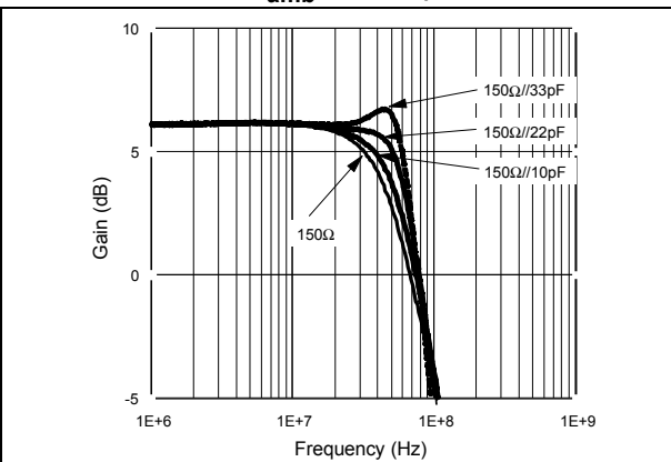
Figure 33. Overshoot function of output capacitance (gain = +2, V_{CC} = \pm 5\text{ V} , T_{amb} = 25\text{ }^\circ\text{C} )
