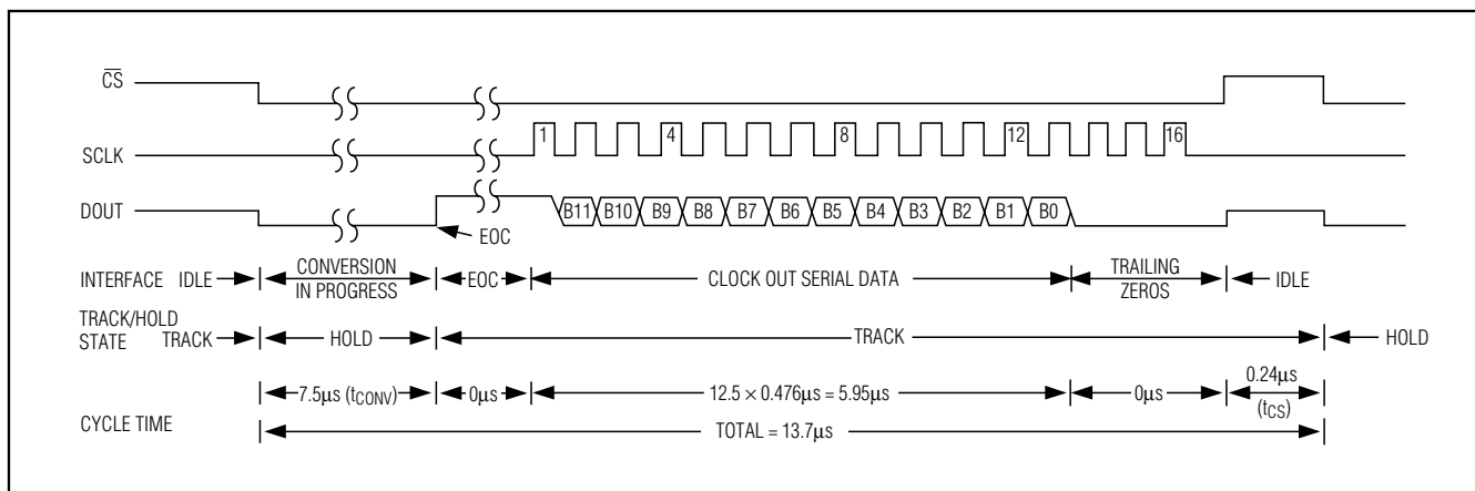
Figure 8. Interface Timing Sequence
