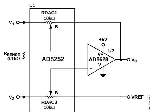
Figure 45. Current-Sensing Amplifier
