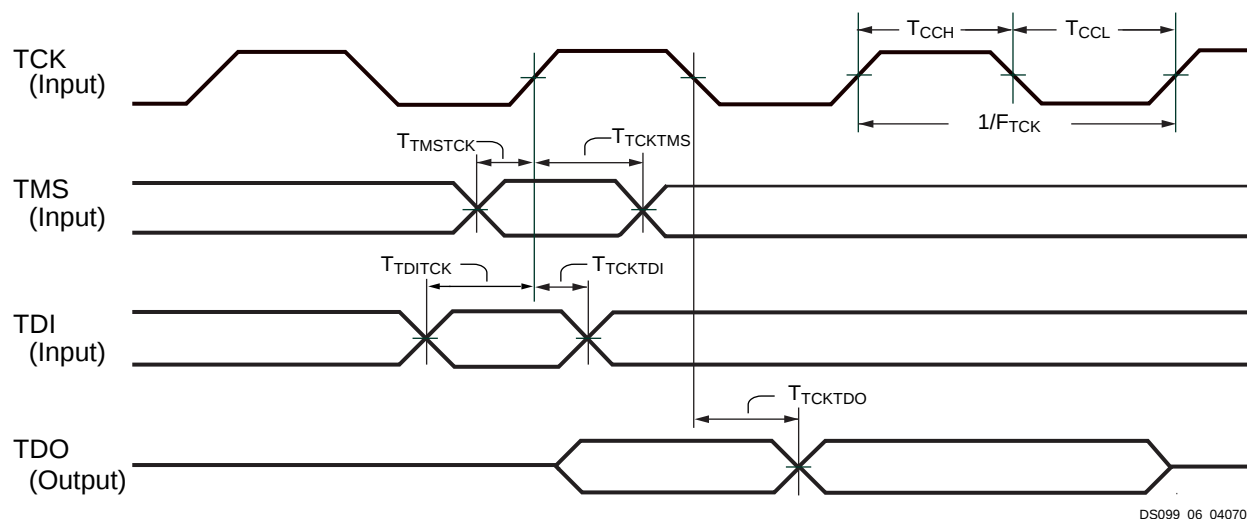
Figure 37: JTAG Waveforms
