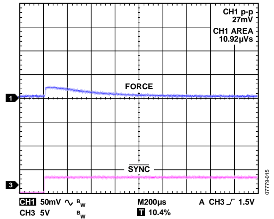
Figure 29. Range Change 2.5 mA to 25 mA, Safe Mode, 2.5 mA I_{LOAD} , 10 \mu F Load
