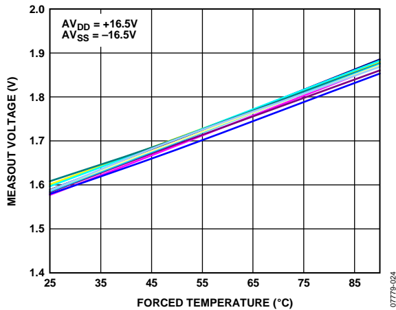
Figure 38. MEASOUT TSENSE Temperature Sensor vs. Temperature (Multiple Devices)
