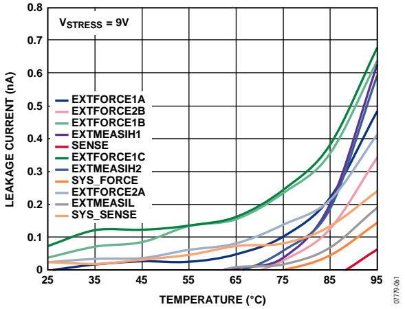
Figure 20. Leakage Current vs. Temperature, V_{STRESS} = 9V
