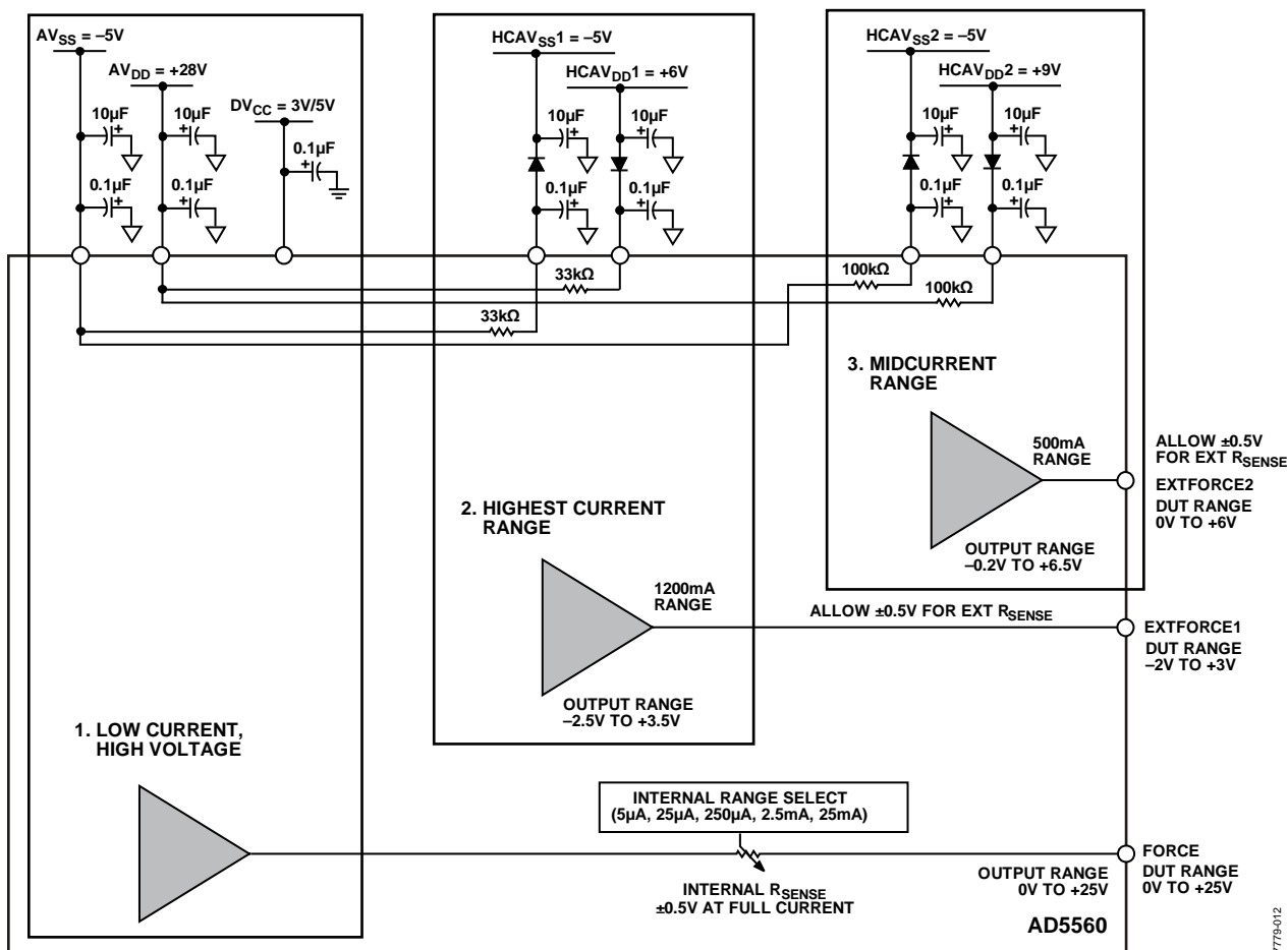
Figure 57. Example of Using the Extra Supply Rails Within the AD5560 to Achieve Multiple Voltage/Current Ranges
