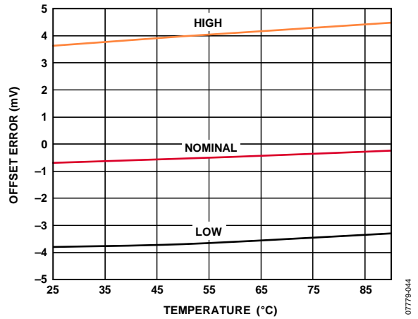
Figure 28. MV Offset Error vs. Temperature, MEASOUT Gain = 0.2
