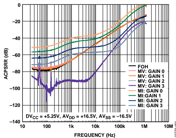
Figure 48. ACPSRR of AVSS vs. Frequency
