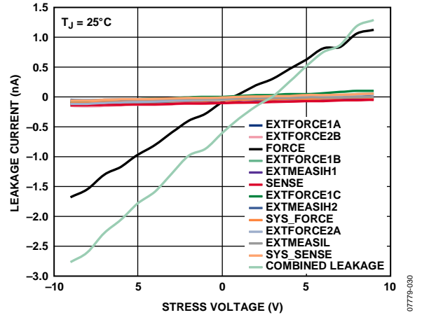
Figure 17. Leakage Current vs. Stress Voltage (Force and Combined Leakage)
