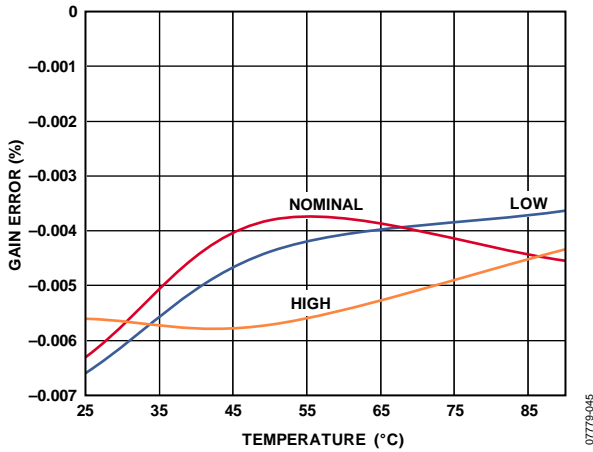
Figure 25. MV Gain Error vs. Temperature, MEASOUT Gain = 1
