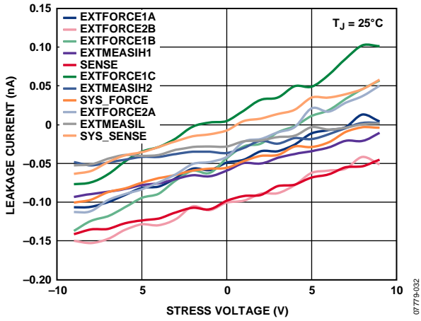
Figure 19. Leakage Current vs. Stress Voltage
