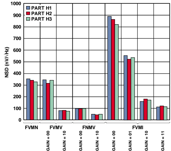
Figure 46. NSD vs. Amplifier Stage and Gain Setting at 1 kHz
