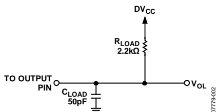
Figure 2. Load Circuit for Open Drain
