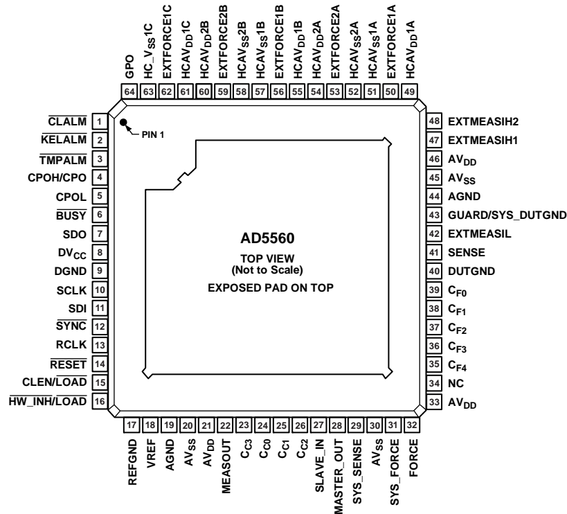
Figure 6. Pin Configuration
