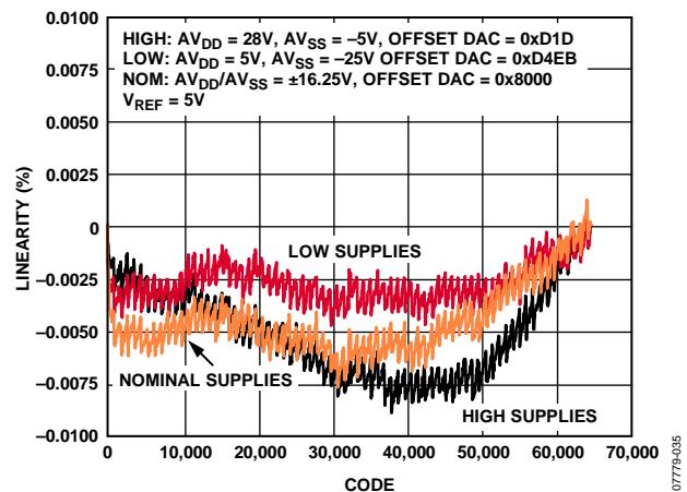
Figure 11. Measure Current Linearity vs. Code (MEASOUT Gain = 1, MI Gain = 20), T_j = 25^\circ\text{C}
