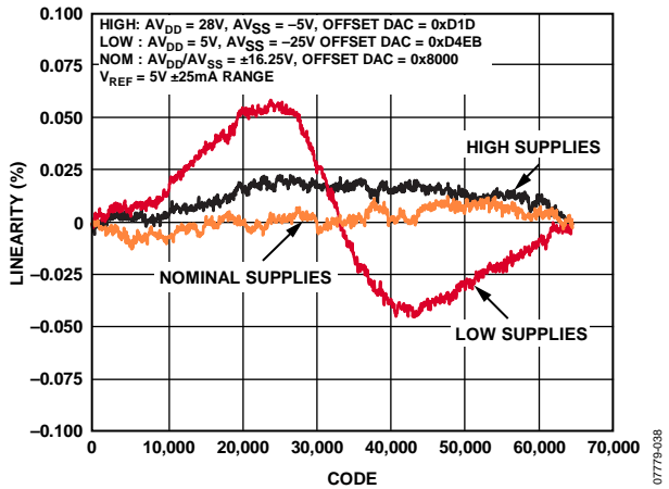
Figure 14. Measure Current Linearity vs. Code (MEASOUT Gain = 0.2, MI Gain = 10)
