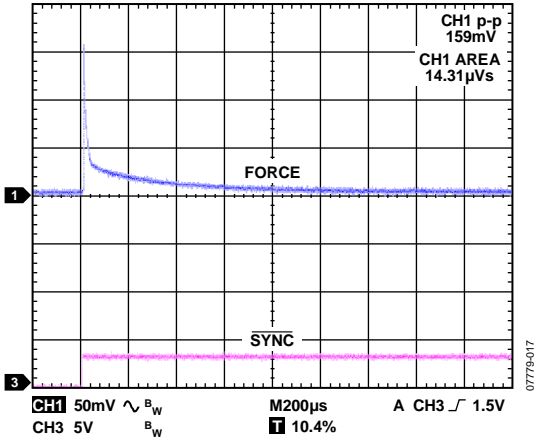
Figure 31. Range Change 25 mA to EXTFORCE2, Safe Mode, 25 mA I_{LOAD} , 10 µF Load
