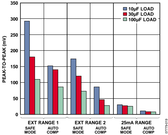
Figure 33. Kick/Droop Response vs. I_{RANGE} , Compensation, and C_{LOAD} , 10% to 90% to 10% I_{LOAD} Change
