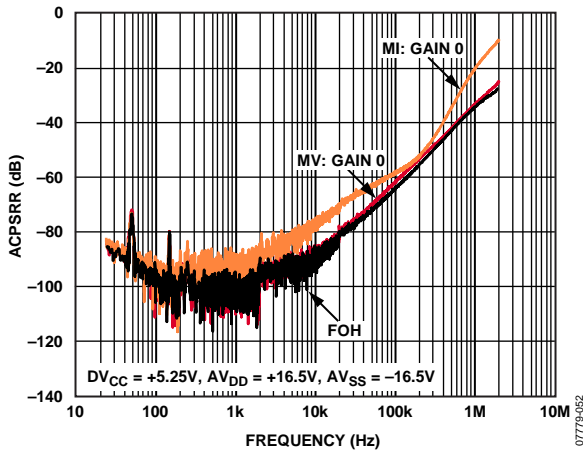
Figure 50. ACPSRR of HCAV DDx vs. Frequency
