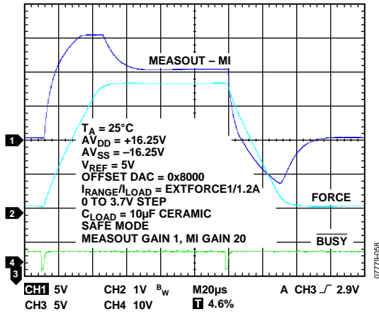
Figure 43. Transient Response FVMI Mode, EXTFORCE1 Range, Safe Mode
