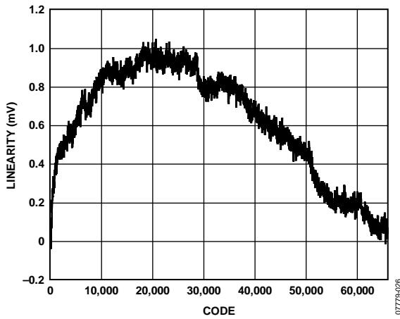
Figure 7. Force Voltage Linearity vs. Code, V_{REF} = 5V , No Load
