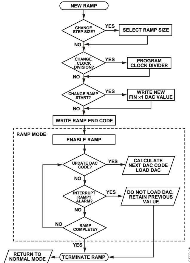
Figure 56. Flow Chart for Ramp Function
