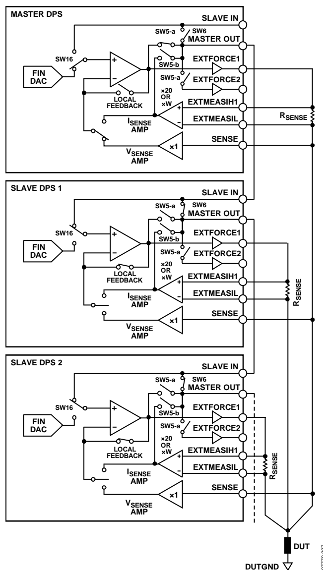
Figure 52. Simplified Block Diagram of High Current Ganging Mode
