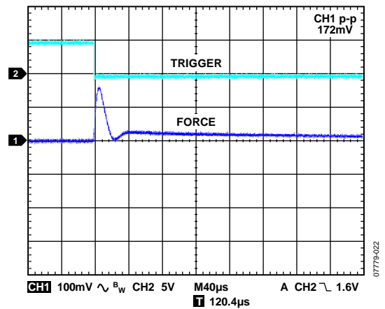
Figure 36. Safe Mode 80% to 10%, EXTFORCE2 Range, 10 µF Load
