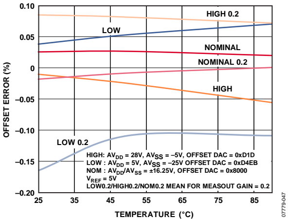
Figure 21. MI Offset Error vs. Temperature, MI Gain = 20, MEASOUT Gain = 1 and 0.2
