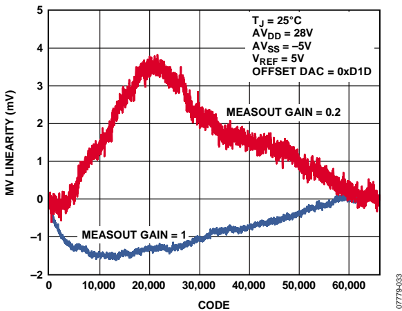
Figure 9. Measure Voltage Linearity vs. Code (MEASOUT Gain = 1, MEASOUT Gain = 0.2, Positive Skew Supply)
