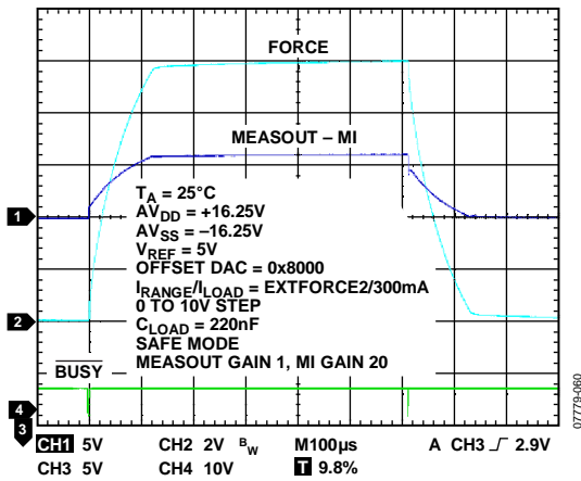
Figure 45. Transient Response FVMI Mode, EXTFORCE2 Range, Safe Mode
