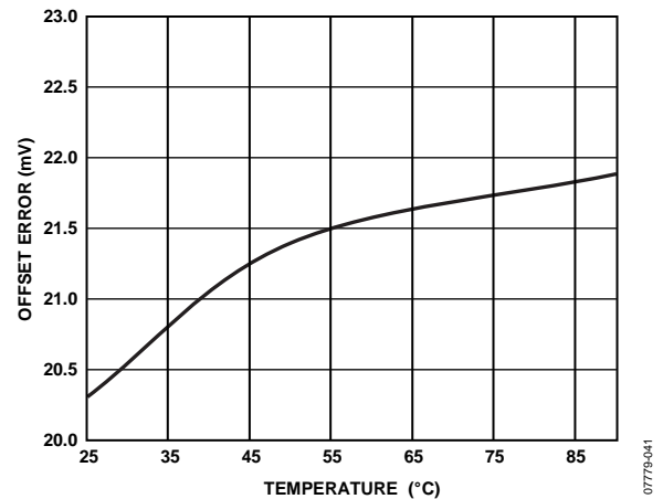
Figure 24. FV Offset Error vs. Temperature
