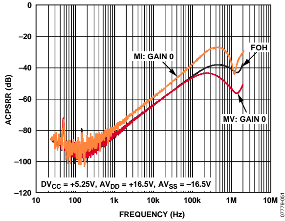
Figure 49. ACPSRR of DV CC vs. Frequency
