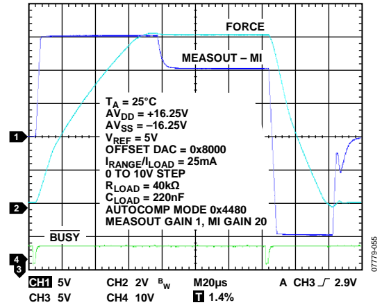
Figure 40. Transient Response FVMI Mode, 25 mA Range, Autocompensation Mode
