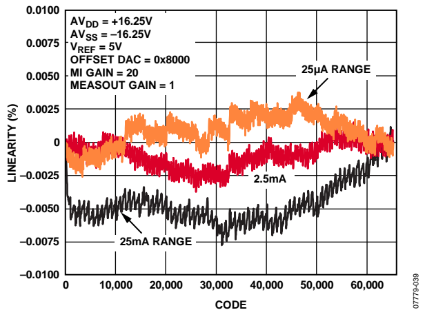
Figure 15. Measure Current Linearity vs. I_{RANGE} (MEASOUT Gain = 1, MI Gain = 20)
