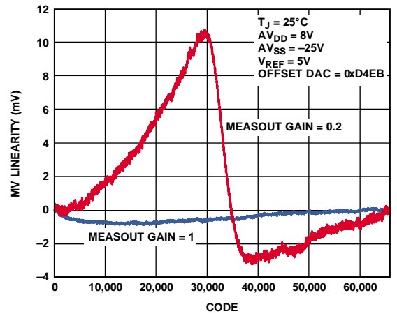
Figure 10. Measure Voltage Linearity vs. Code (MEASOUT Gain 1, MEASOUT Gain = 0.2, Negative Skew Supply)
