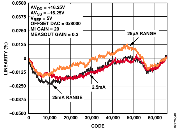
Figure 16. Measure Current Linearity vs. I_{RANGE} (MEASOUT Gain = 0.2, MI Gain = 20)
