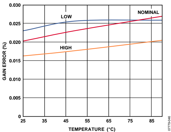
Figure 27. MV Gain Error vs. Temperature, MEASOUT Gain = 0.2
