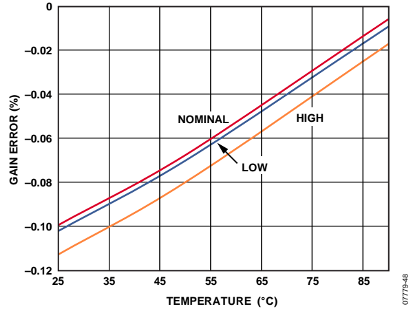
Figure 22. MI Positive Gain Error vs. Temperature, MI Gain = 20, MEASOUT Gain = 1
