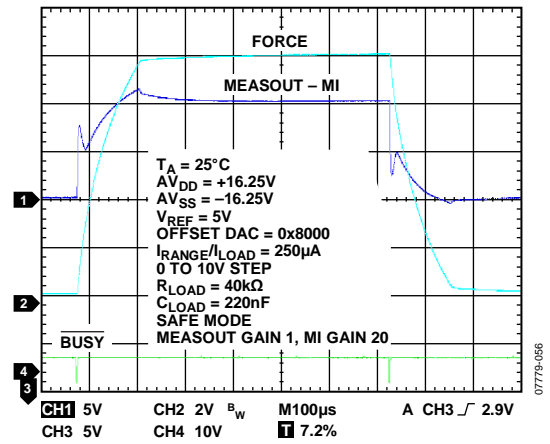
Figure 41. Transient Response FVMI Mode, 25mA Range, Safe Mode
