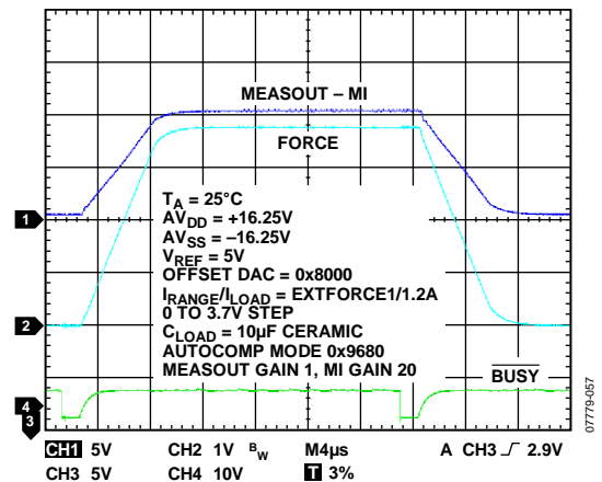
Figure 42. Transient Response FVMI Mode, EXTFORCE1 Range, Autocompensation Mode
