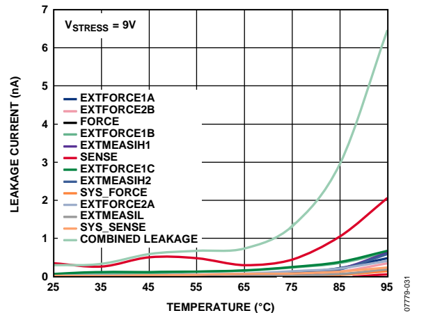
Figure 18. Leakage Current vs. Temperature (Force and Combined Leakage), V_{STRESS} = 9V
