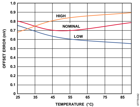
Figure 26. MV Offset Error vs. Temperature, MEASOUT Gain = 1
