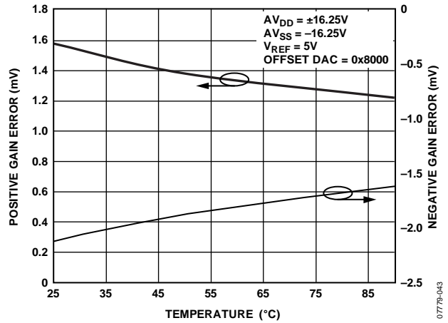
Figure 23. FV Gain Error vs. Temperature
