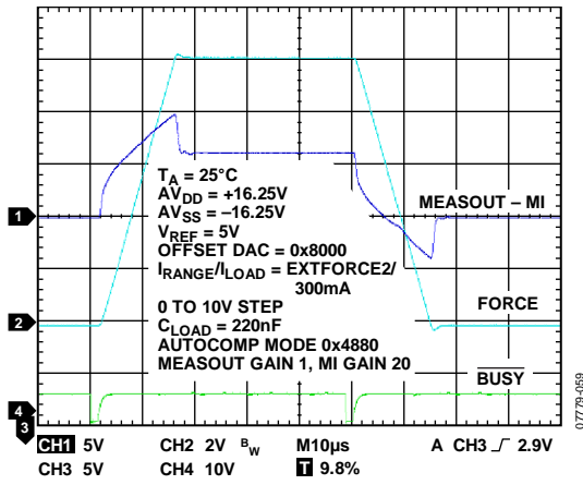
Figure 44. Transient Response FVMI Mode, EXTFORCE2 Range, Autocompensation Mode
