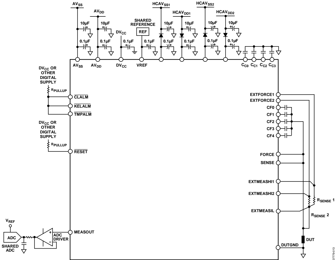
Figure 58. External Components Required for Use with the DPS
