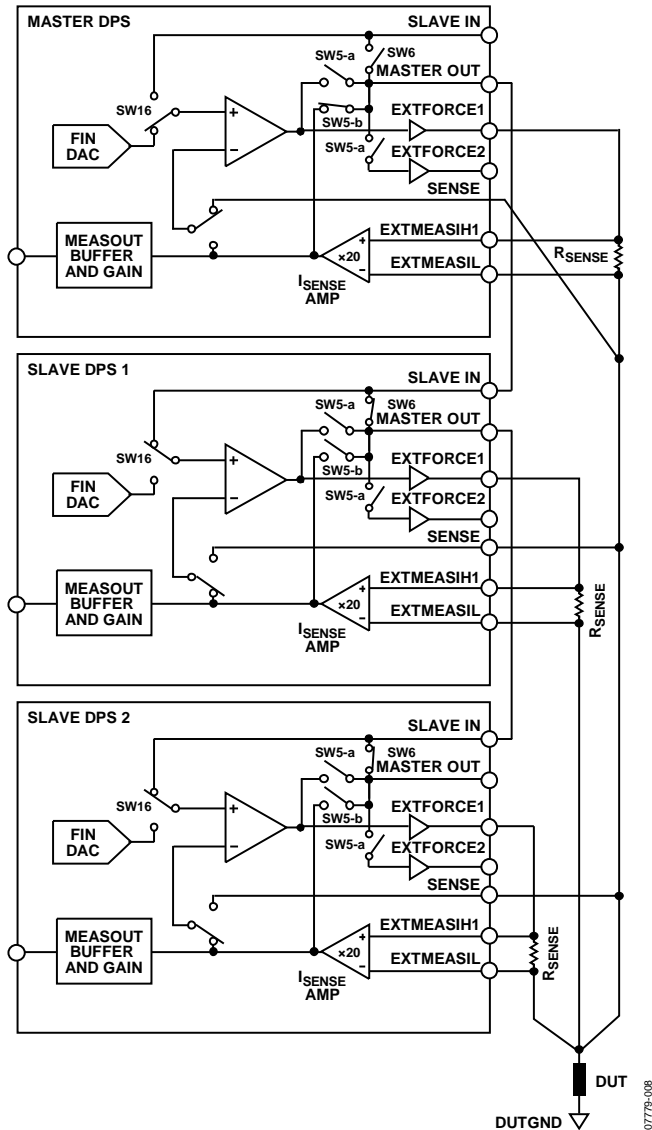
Figure 53. Simplified Block Diagram of Gang Mode, Using an FV/FI Combination
