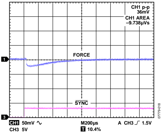
Figure 32. Range Change EXTFORCE2 to 25 mA, Safe Mode, 25 mA I_{LOAD} , 10 µF Load
