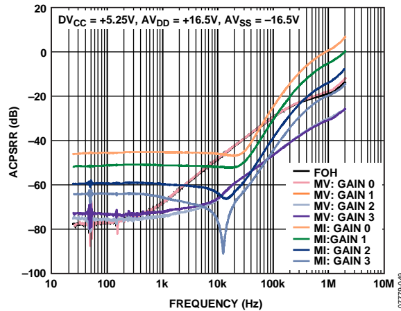
Figure 47. ACPSRR of AVDD vs. Frequency
