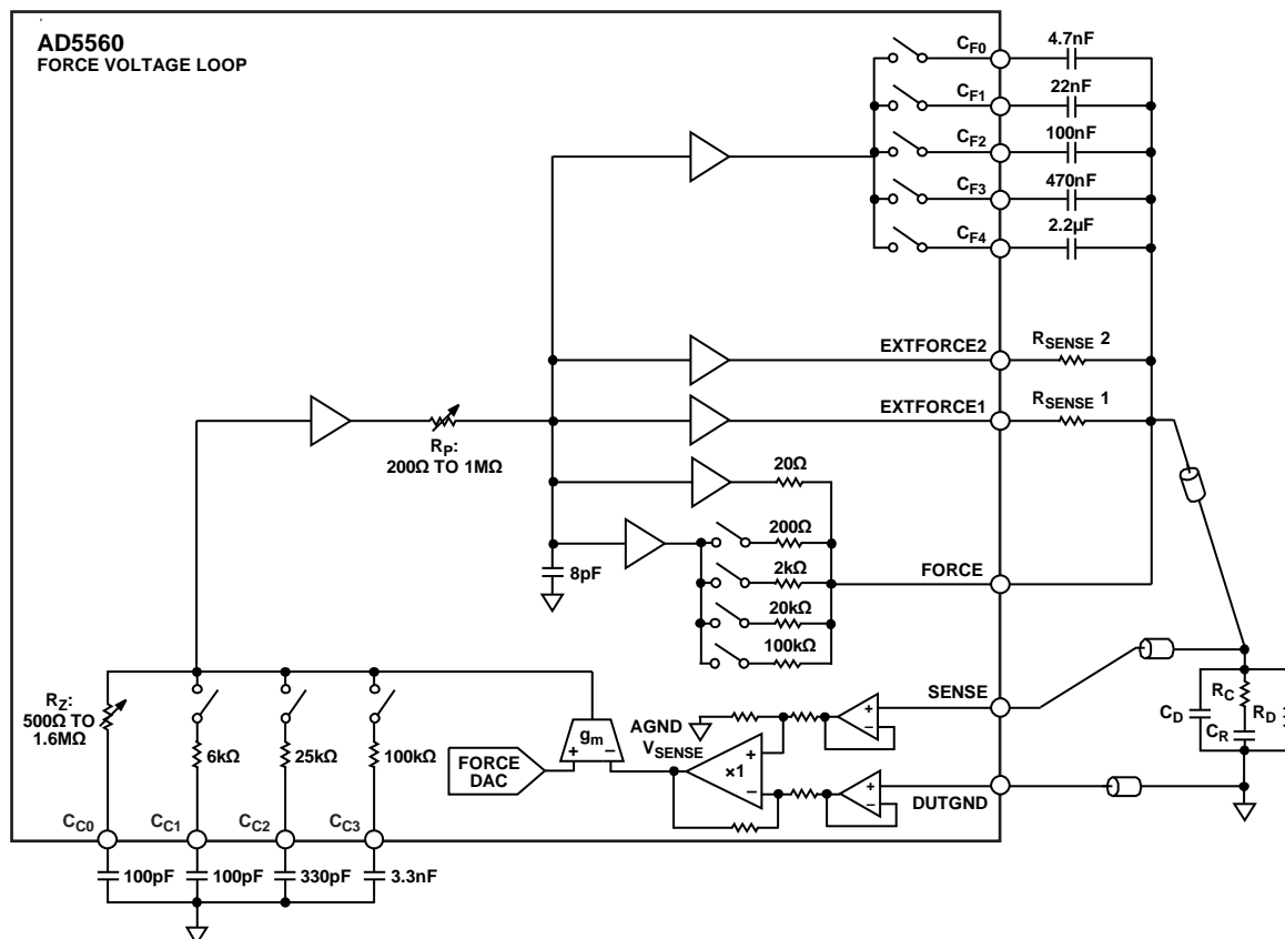
Figure 55. Block Diagram of a Force Amplifier Loop
