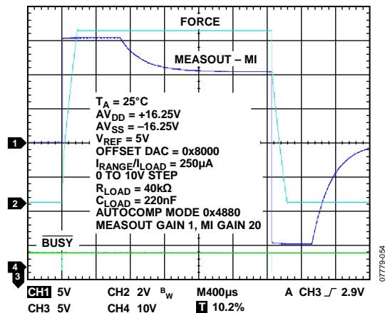
Figure 39. Transient Response FVMI Mode, \pm 250 \mu\text{A} Range, Autocompensation Mode
