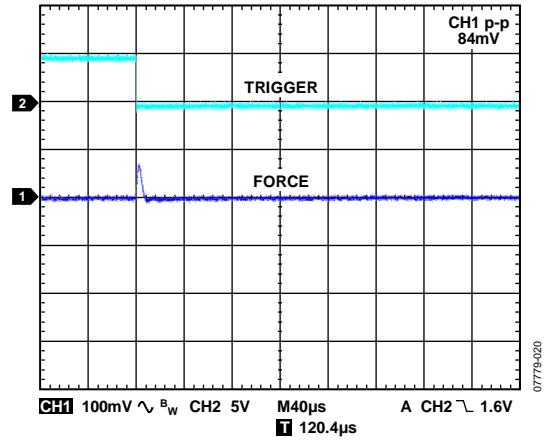
Figure 34. Autocompensation Mode 90% to 10% I_{LOAD} Change, EXTFORCE2 Range, 10 µF Load
