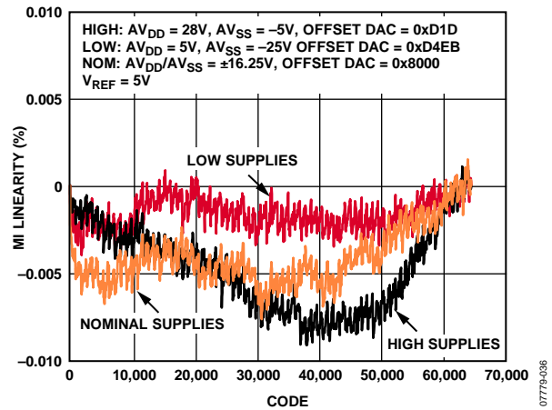
Figure 12. Measure Current Linearity vs. Code (MEASOUT Gain = 1, MI Gain = 10)
