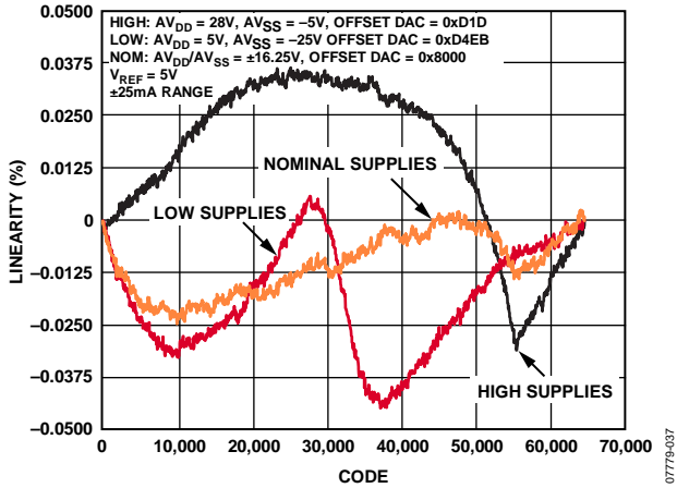
Figure 13. Measure Current Linearity vs. Code (MEASOUT Gain = 0.2, MI Gain = 20)
