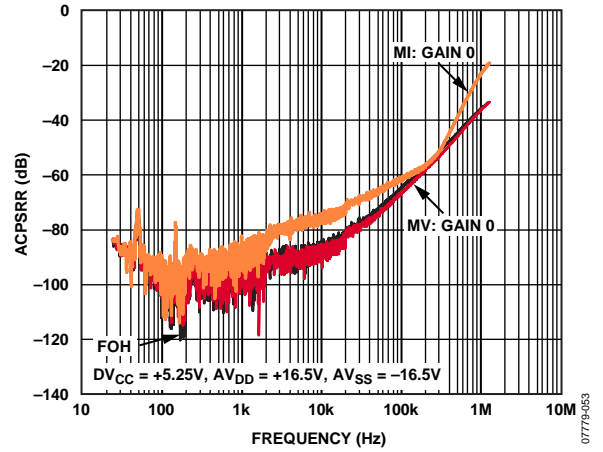
Figure 51. ACPSRR of HCAV SSx vs. Frequency
