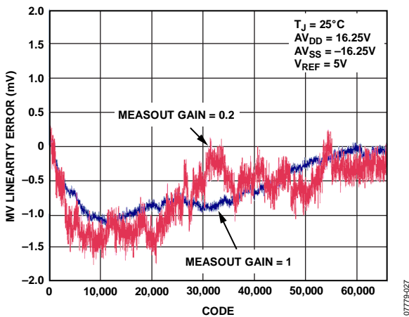
Figure 8. Measure Voltage Linearity vs. Code (MEASOUT Gain = 1, MEASOUT Gain = 0.2, Nominal Supplies)
