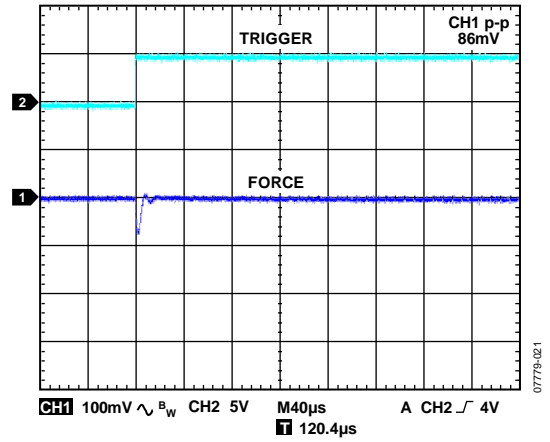
Figure 35. Autocompensation Mode 10% to 90% I_{LOAD} Change, EXTFORCE2 Range, 10 µF Load
