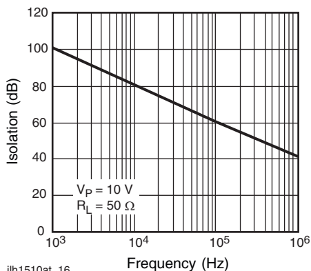
Fig. 17 - Output Isolation
