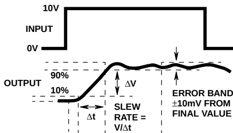
FIGURE 3. SETTLING TIME
