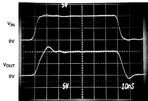
+10V RESPONSE
