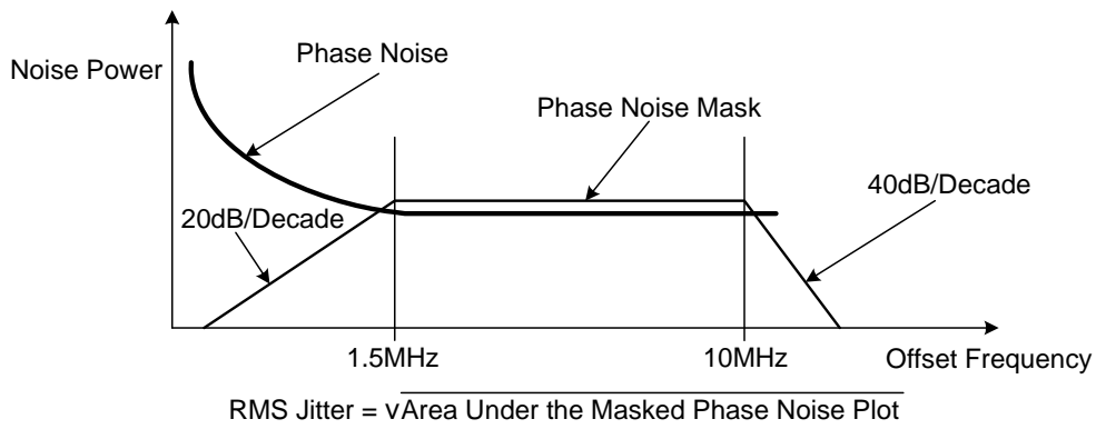
Figure 3. RMS Phase Jitter
