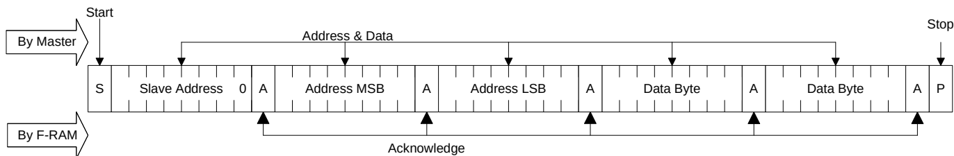
Figure 18. Multi-Byte Write
