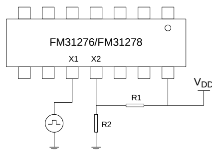
Figure 10. External Oscillator
