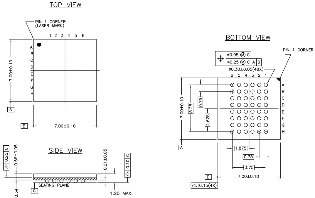
Figure 12. 48-ball FBGA (7 × 7 × 1.2 mm) BA48 Package Outline, 51-85096
