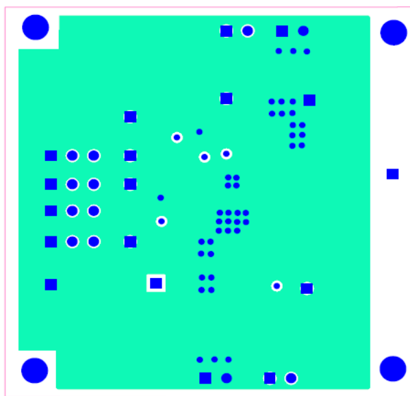
Figure 18. 2 nd Layer
