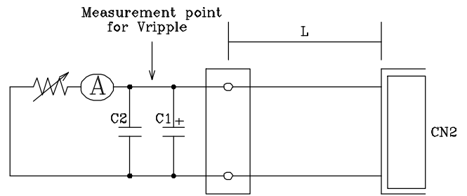
Fig.A L:150mmAWG#18x2 C1:Elec.Cap 100uF C2:Film Cap 1uF Bandwidth of scope:100MHz
