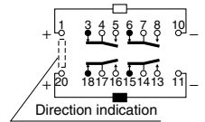
2-coil latching
