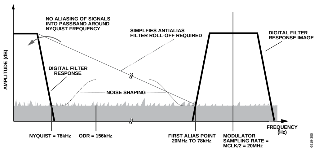
Figure 27. Antialias Example Using the AD7765 in Normal Mode, Decimate 128× Using MCLK/2 = ICLK = 20\text{ MHz}
