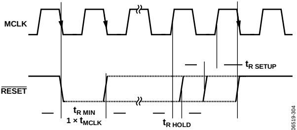
Figure 38. RESET Timing Synchronous to MCLK
