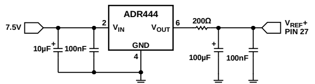
Figure 46. Reference Connection
