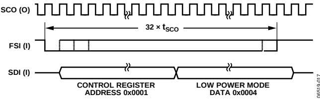
Figure 37. Write Scheme for Low Power Mode
