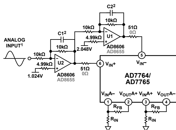
Figure 34. Driving the AD7765 Modulator Inputs Directly from a Single-Ended Source (On-Board Differential Amplifier Powered Down)
