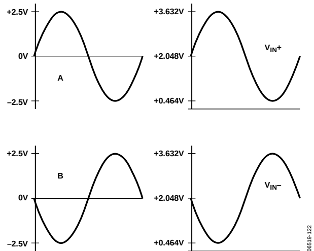
Figure 30. Differential Amplifier Signal Conditioning
