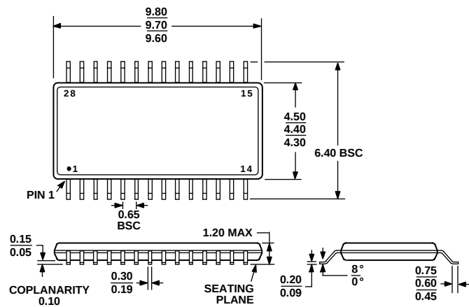
COMPLIANT TO JEDEC STANDARDS MO-153-AE Figure 48. 28-Lead Thin Shrink Small Outline Package [TSSOP] (RU-28) Dimensions shown in millimeters
