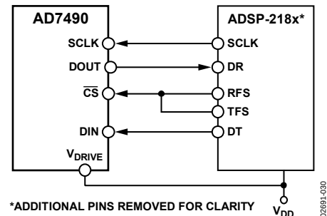
Figure 31. Interfacing to the ADSP-218x
