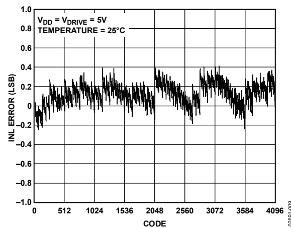
Figure 10. Typical INL
