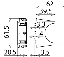
Dimension drawing DG PCB NPE FM
