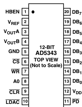
AD5343 PIN CONFIGURATION
