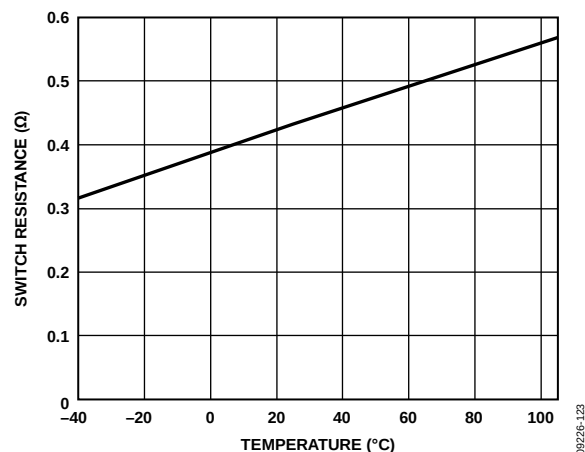
Figure 60. Switch Resistance vs. Temperature
