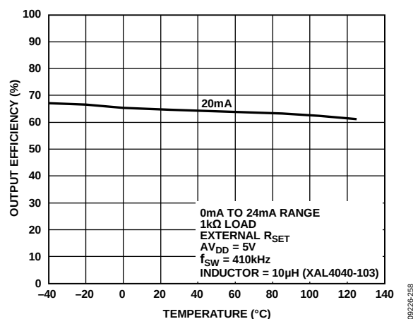
Figure 59. Output Efficiency vs. Temperature (See Figure 81)
