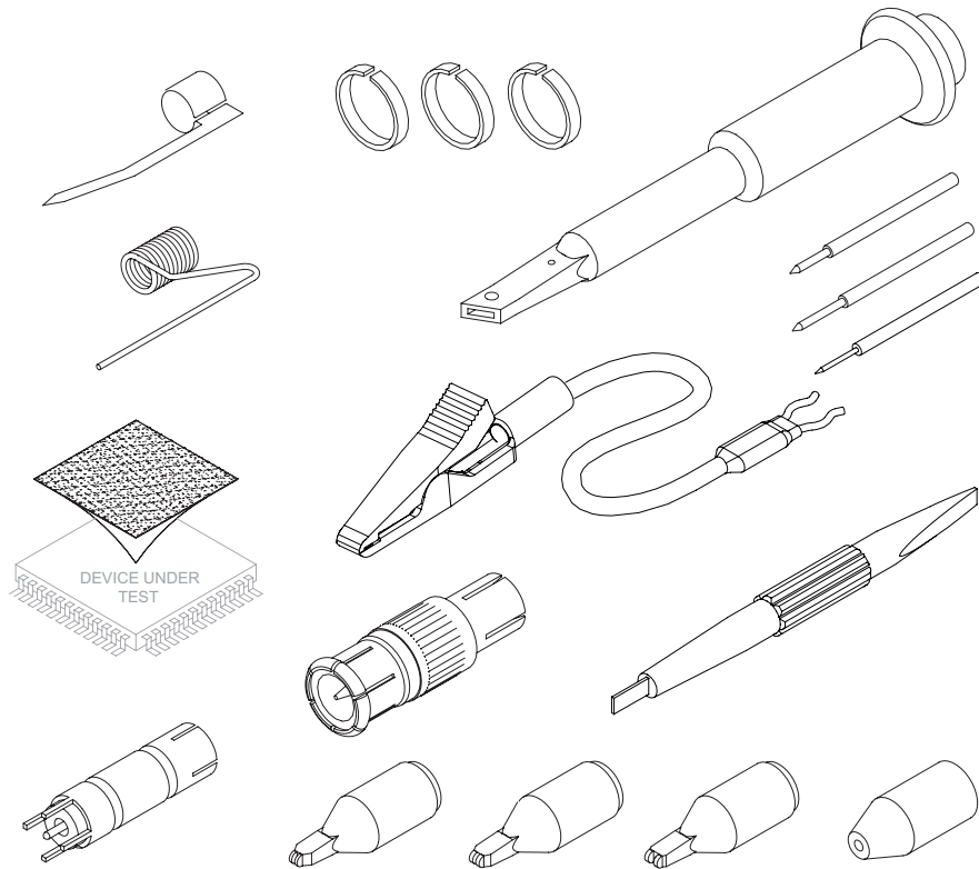
Comprehensive set of accessories for 5.0 mm PMK probes.
