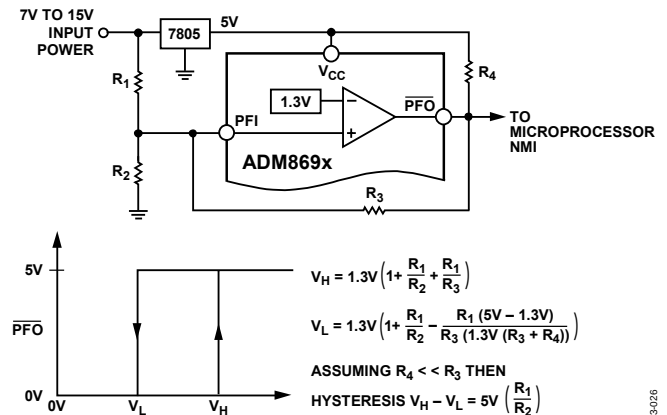
Figure 26. Adding Hysteresis to the Power-Fail Comparator
