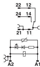
AC coils
