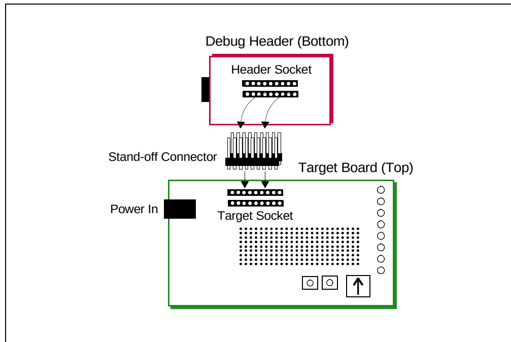
FIGURE 5: CONNECT HEADER TO TARGET
