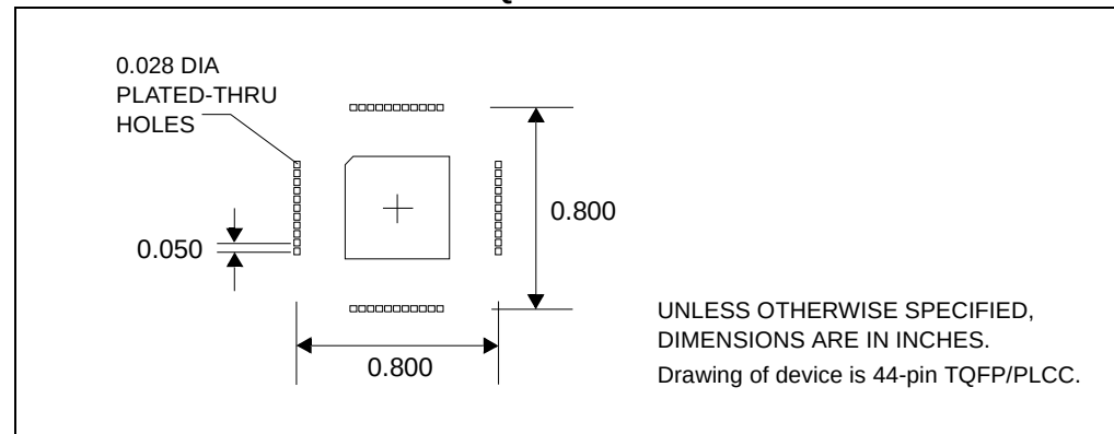
FIGURE 2: SINGLE-ROW TQFP/PLCC FOOTPRINT
