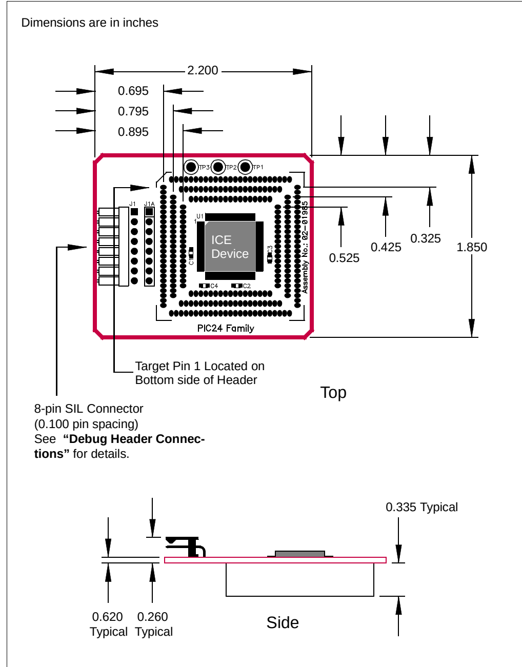
FIGURE 5: DIMENSIONS – AC244022
