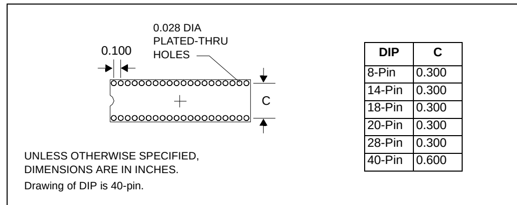
FIGURE 1: DIP FOOTPRINT
