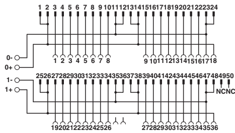
Connection scheme: FLKM 50-PA-AB/1756/EXTC
