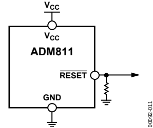
Figure 11. Ensuring a Valid \overline{RESET} Output Down to V_{CC} = 0 V
