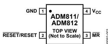
Figure 3. Pin Configuration
