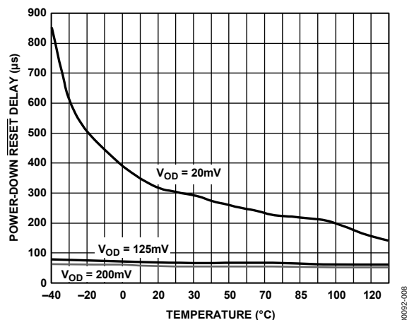
Figure 8. Power-Down \overline{\text{RESET}} Delay vs. Temperature (ADM81xL/M)
