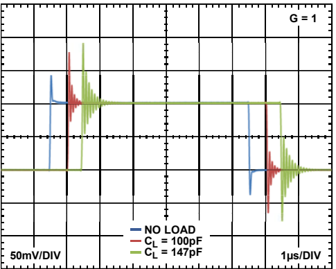
Figure 39. Small Signal Response with Various Capacitive Loads ( G = 1 ), R_L = \text{Infinity}
