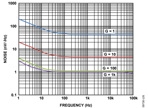
Figure 26. RTI Voltage Noise Spectral Density vs. Frequency
