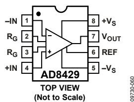
Figure 48. Pinout Diagram
