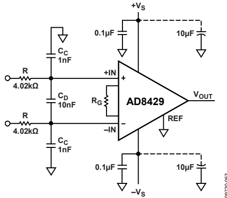
Figure 53. RFI Suppression
