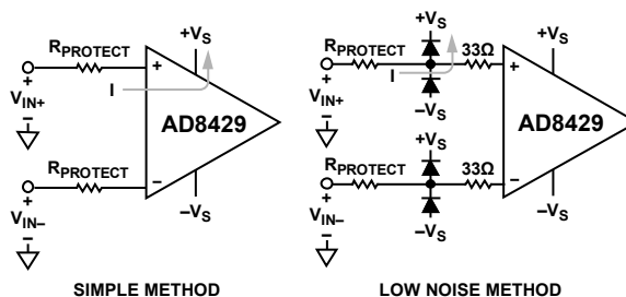
Figure 51. Protection for Voltages Beyond the Rails
