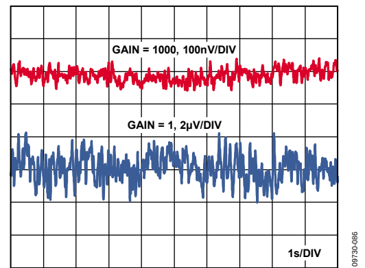
Figure 27. 0.1 Hz to 10 Hz RTI Voltage Noise ( G = 1 , G = 1000 )
