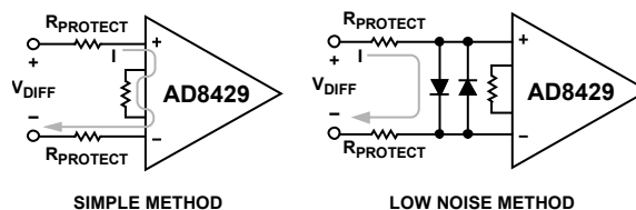
Figure 52. Protection for Large Differential Voltages
